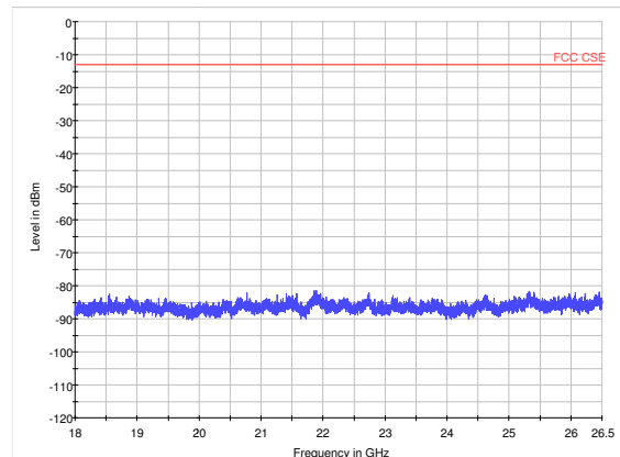
LTE Band 41 10MHz CH41185 18GHz~26.5GHz
