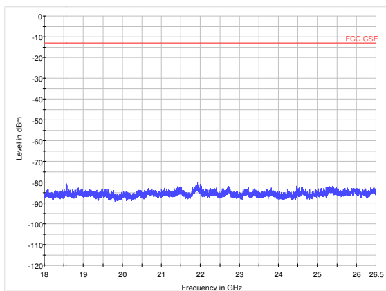
LTE Band 41 5MHz CH41215 18GHz~26.5GHz
