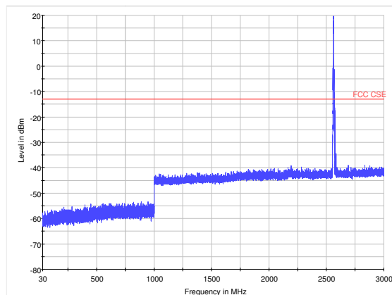
LTE Band 41 20MHz CH40315 30MHz~3GHz
