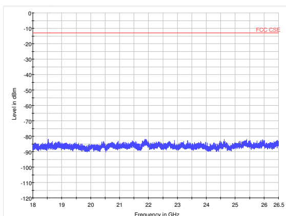
LTE Band 41 15MHz CH41165 18GHz~26.5GHz
