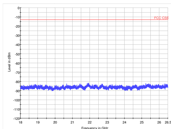
LTE Band 41 5MHz CH40728 18GHz~26.5GHz
