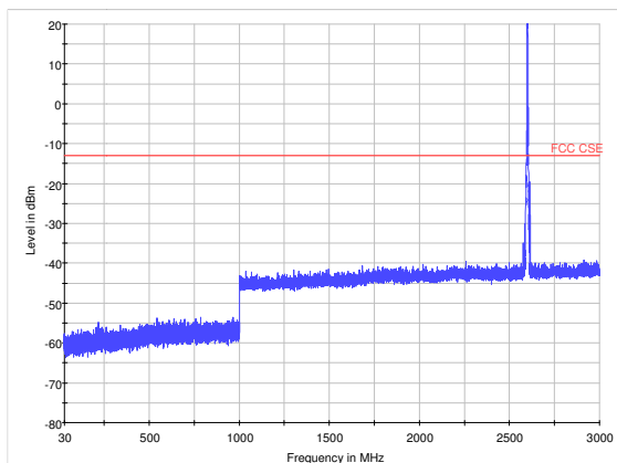
LTE Band 41 20MHz CH40728 30MHz~3GHz
