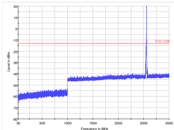
LTE Band 41 5MHz CH40240 30MHz~3GHz
