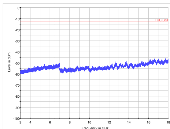
LTE Band 41 5MHz CH40728 3GHz~18GHz
