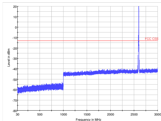
LTE Band 41 15MHz CH40728 30MHz~3GHz
