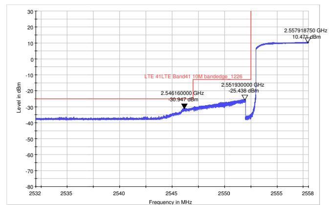
LTE Band 41 QPSK Bandwidth = 10MHz CH40265, RB 50
