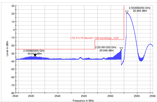
LTE Band 41 QPSK Bandwidth = 10MHz CH40265, RB 1
