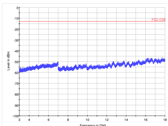
LTE Band 41 15MHz CH40290 3GHz~18GHz
