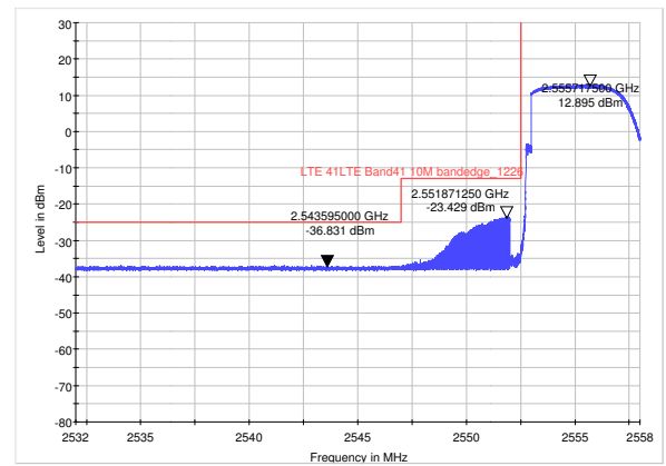
LTE Band 41 QPSK Bandwidth = 10MHz CH40265, RB 50
