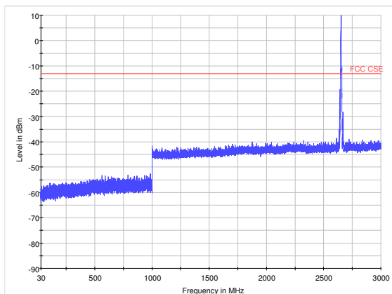
LTE Band 41 5MHz CH41215 30MHz~3GHz
