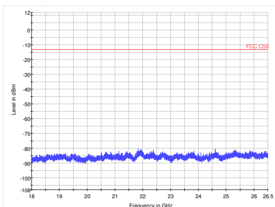
LTE Band 41 5MHz CH40240 18GHz~26.5GHz
