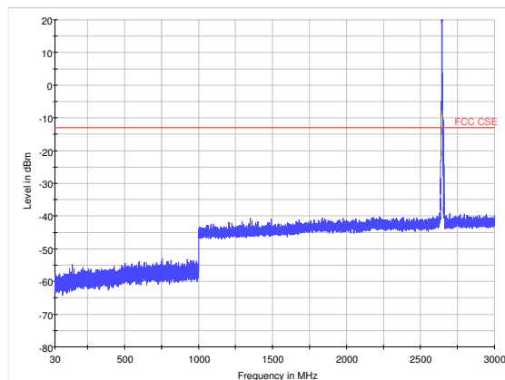
LTE Band 41 20MHz CH41140 30MHz~3GHz
