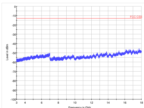
LTE Band 41 15MHz CH41165 3GHz~18GHz
