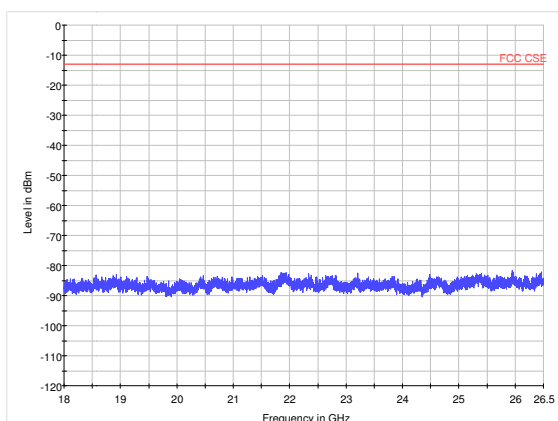
LTE Band 41 15MHz CH40290 18GHz~26.5GHz
