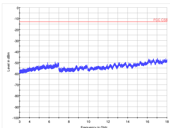
LTE Band 41 20MHz CH40728 3GHz~18GHz
