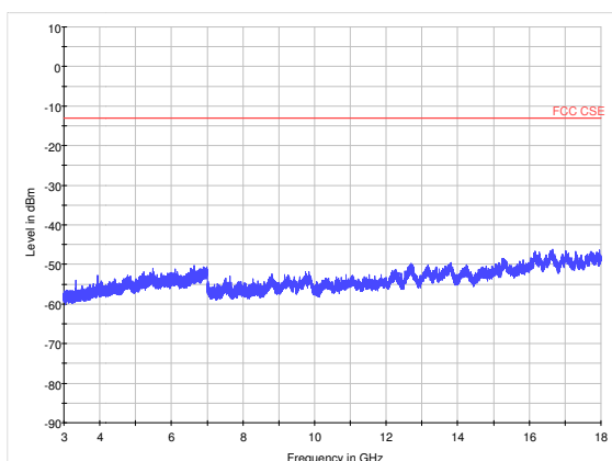
LTE Band 5MHz CH40240 3GHz~18GHz
