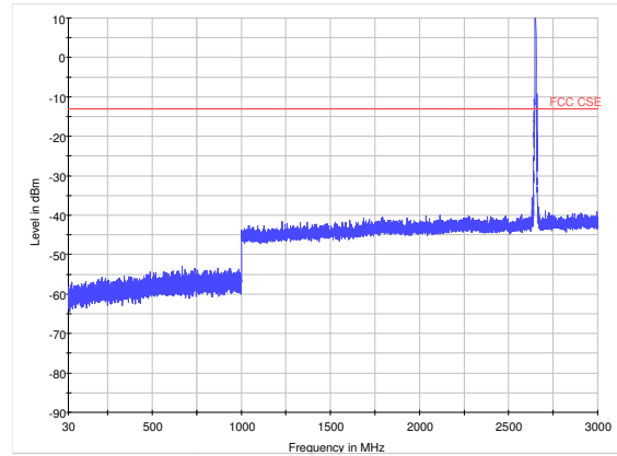
LTE Band 41 10MHz CH41185 30MHz~3GHz
