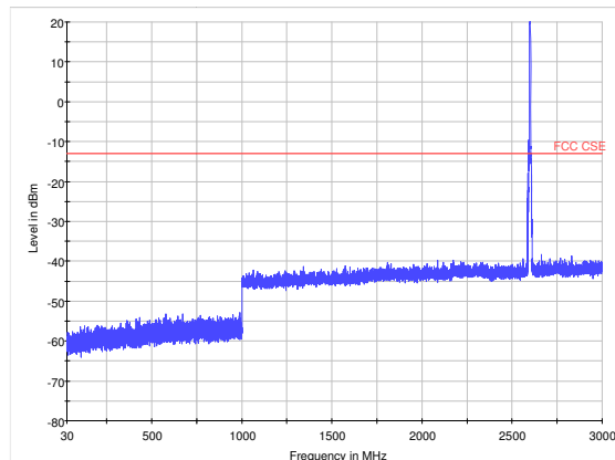
LTE Band 41 5MHz CH40728 30MHz~3GHz
