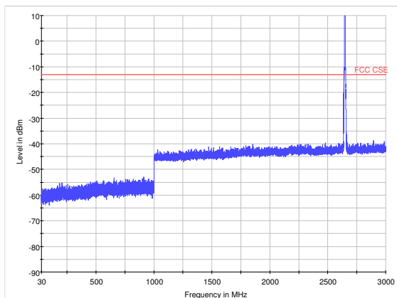
LTE Band 41 15MHz CH41165 30MHz~3GHz
