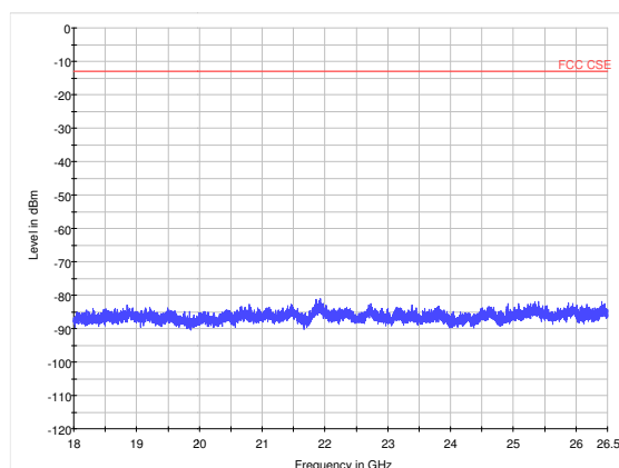
LTE Band 41 15MHz CH40728 18GHz~26.5GHz
