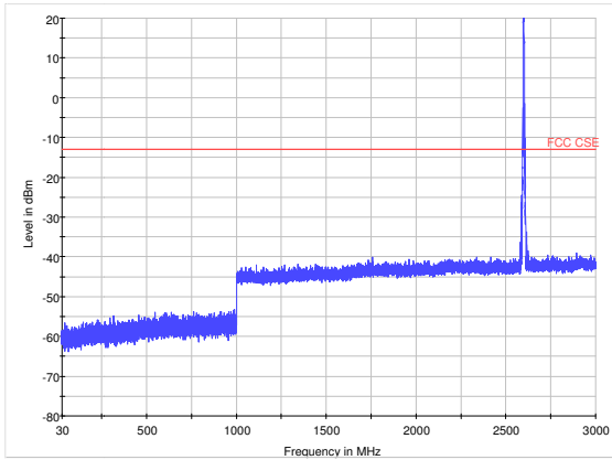
LTE Band 41 10MHz CH40728 30MHz~3GHz
