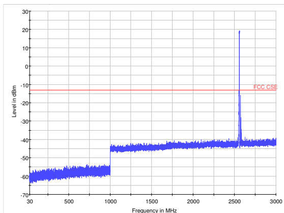
LTE Band 41 15MHz CH40290 30MHz~3GHz
