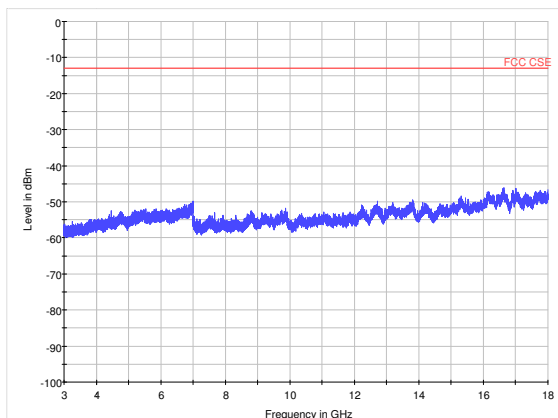
LTE Band 41 5MHz CH41215 3GHz~18GHz
