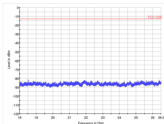
LTE Band 41 20MHz CH41140 18GHz~26.5GHz
