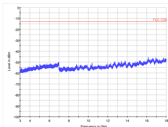
LTE Band 41 15MHz CH40728 3GHz~18GHz
