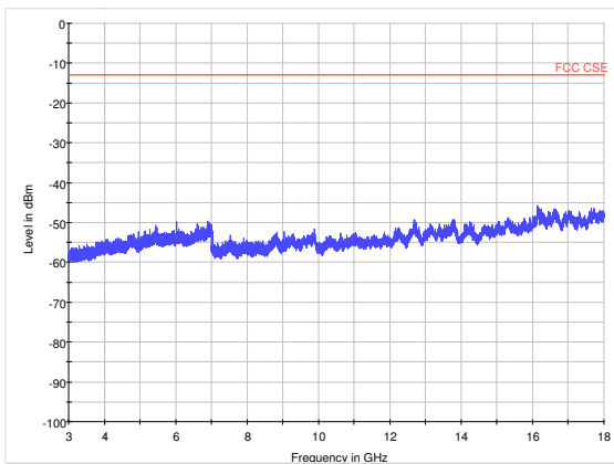
LTE Band 41 10MHz CH40728 3GHz~18GHz
