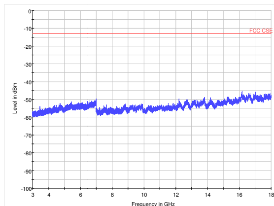
LTE Band 41 10MHz CH40265 3GHz~18GHz
