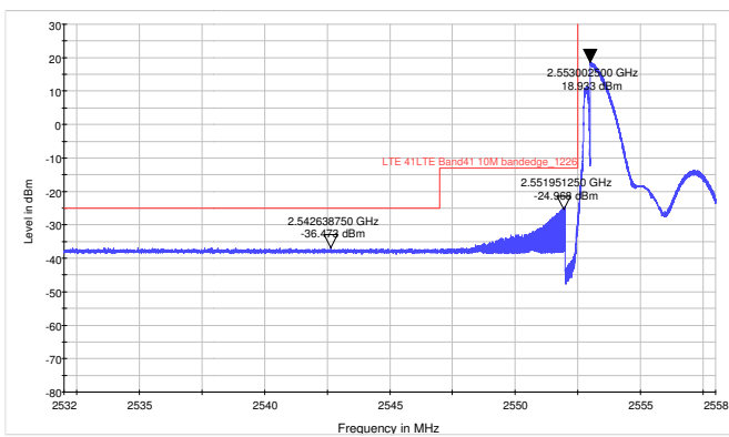
LTE Band 41 QPSK Bandwidth = 10MHz CH40265, RB 1
