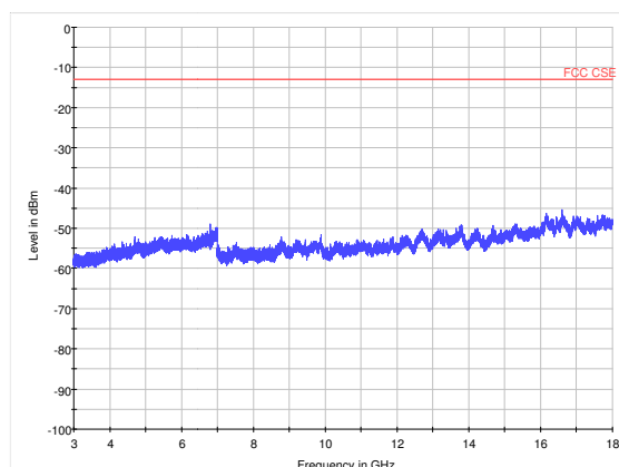
LTE Band 41 20MHz CH40315 3GHz~18GHz
