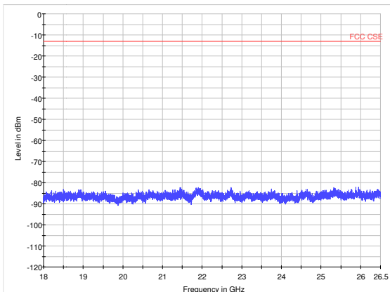
LTE Band 41 10MHz CH40728 18GHz~26.5GHz
