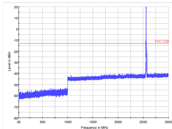
LTE Band 41 10MHz CH40265 30MHz~3GHz
