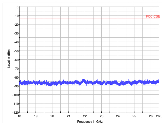
LTE Band 41 10MHz CH40265 18GHz~26.5GHz
