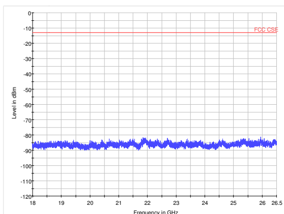
LTE Band 41 20MHz CH40728 18GHz~26.5GHz
