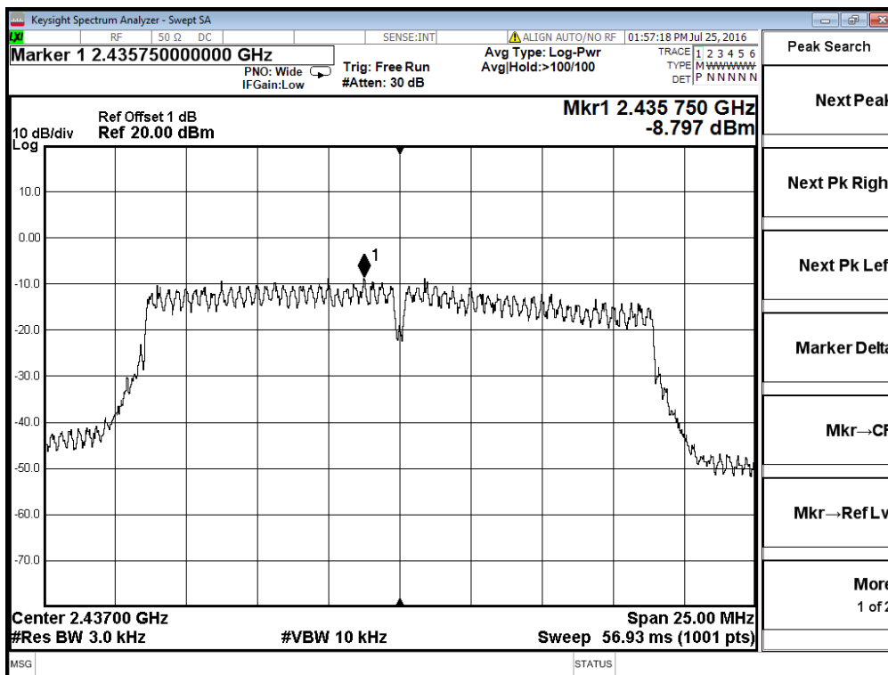
802.11n20 - Channel 6
