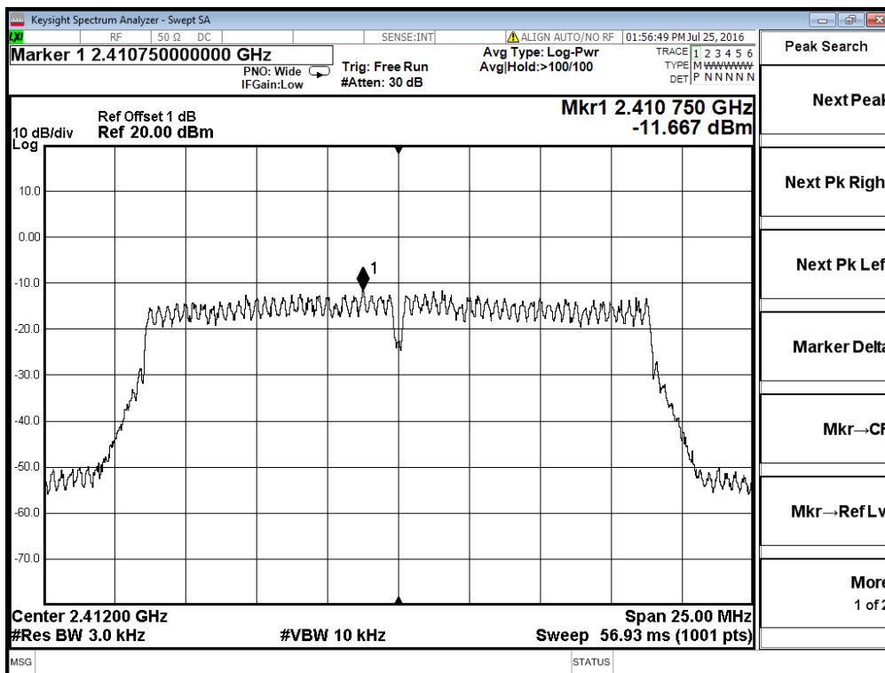
802.11n20 - Channel 1
