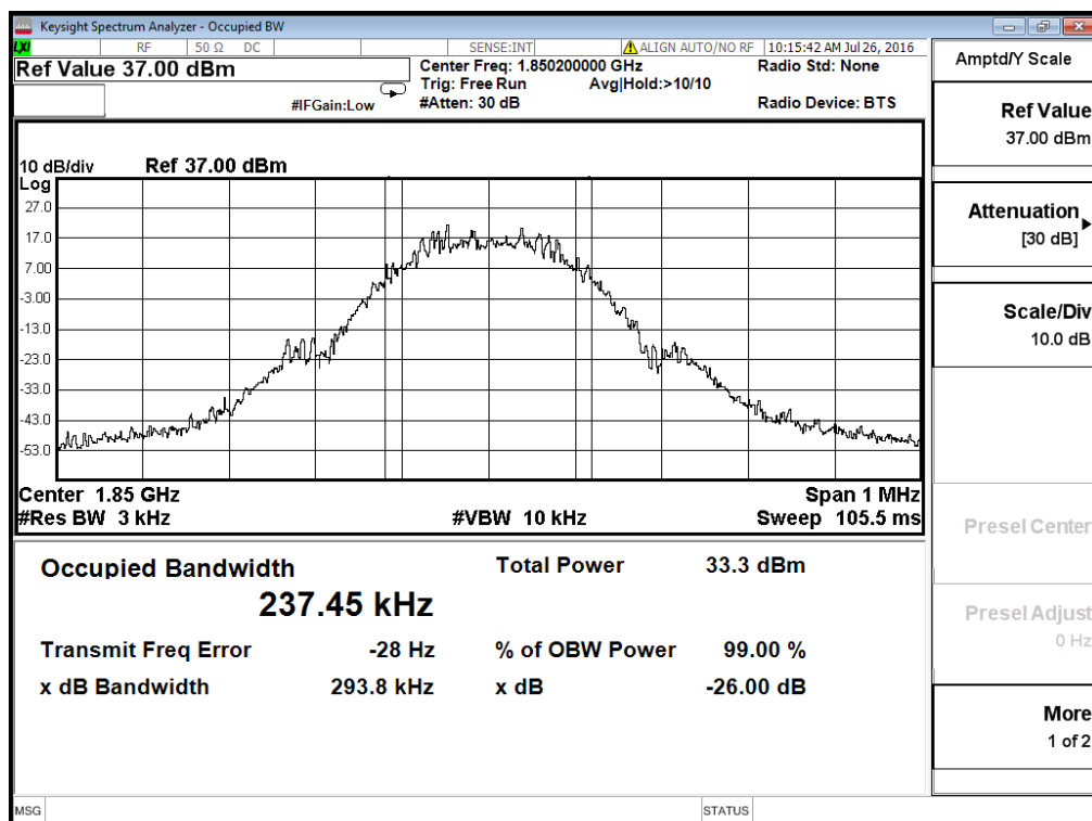
(Plot D1: EDGE 1900MHz Channel = 512 Occupied bandwidth)
