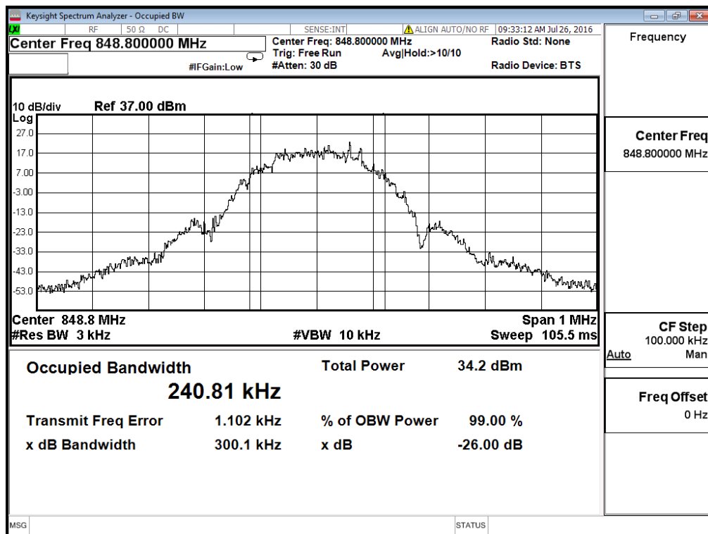
(Plot C3: EDGE 850MHz Channel = 251 Occupied bandwidth)
