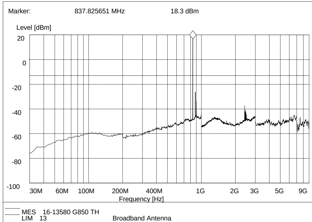
GSM 850MHz, Test Antenna Horizontal
