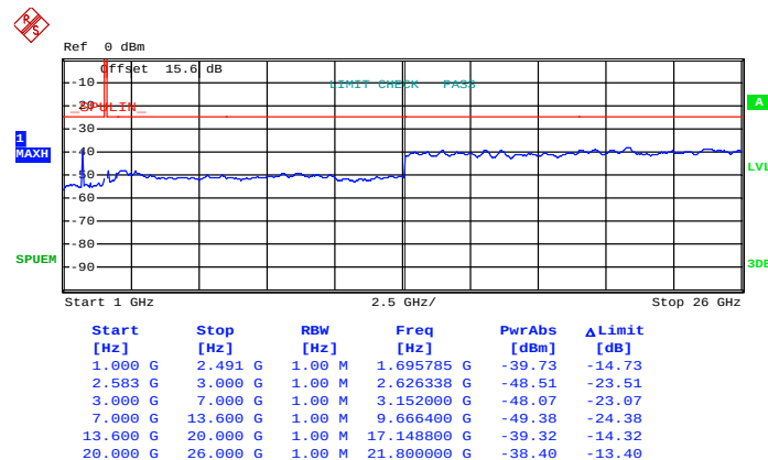
Conducted Emission Plot (1GHz ~ 26GHz) for QPSK (RB Size 1, RB Offset 0)
