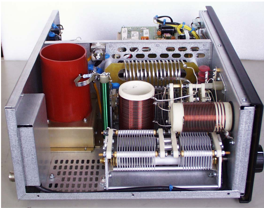
Fig.2 Left side View
