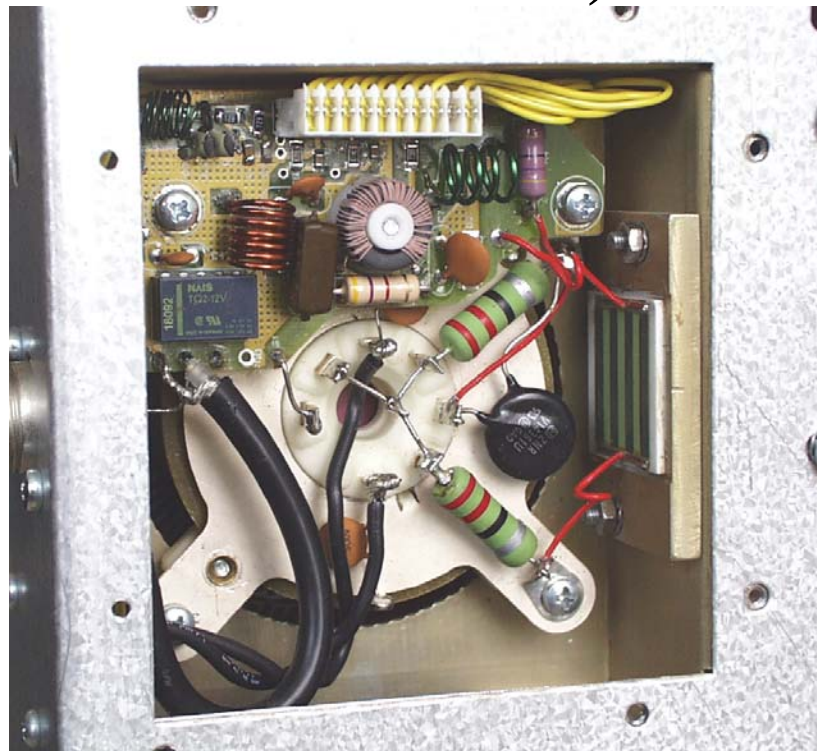
Fig.6 Bottom View – Tube Deck (screen cover removed)
