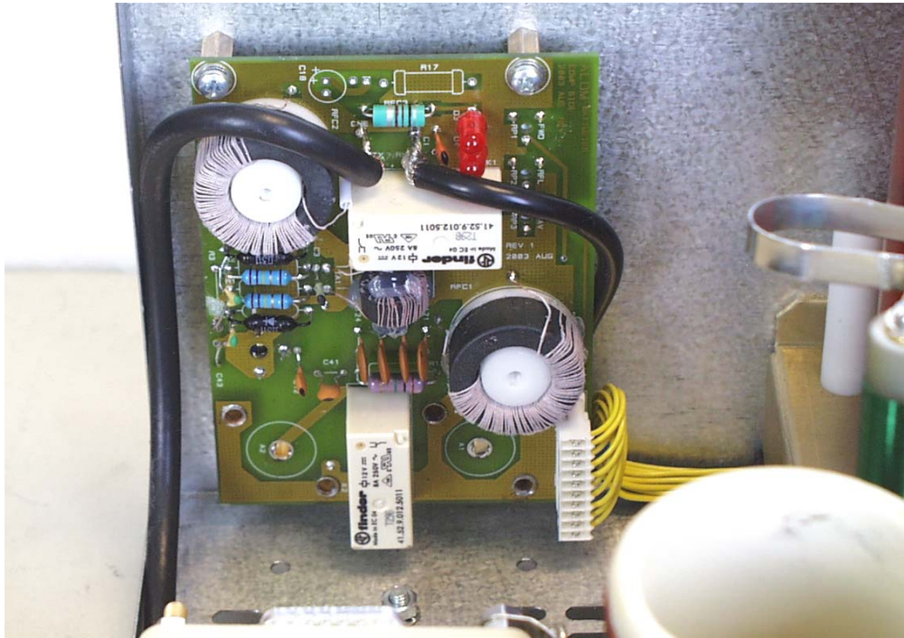
Fig.5 Wattmeter & ant.selection (screen cover removed)
