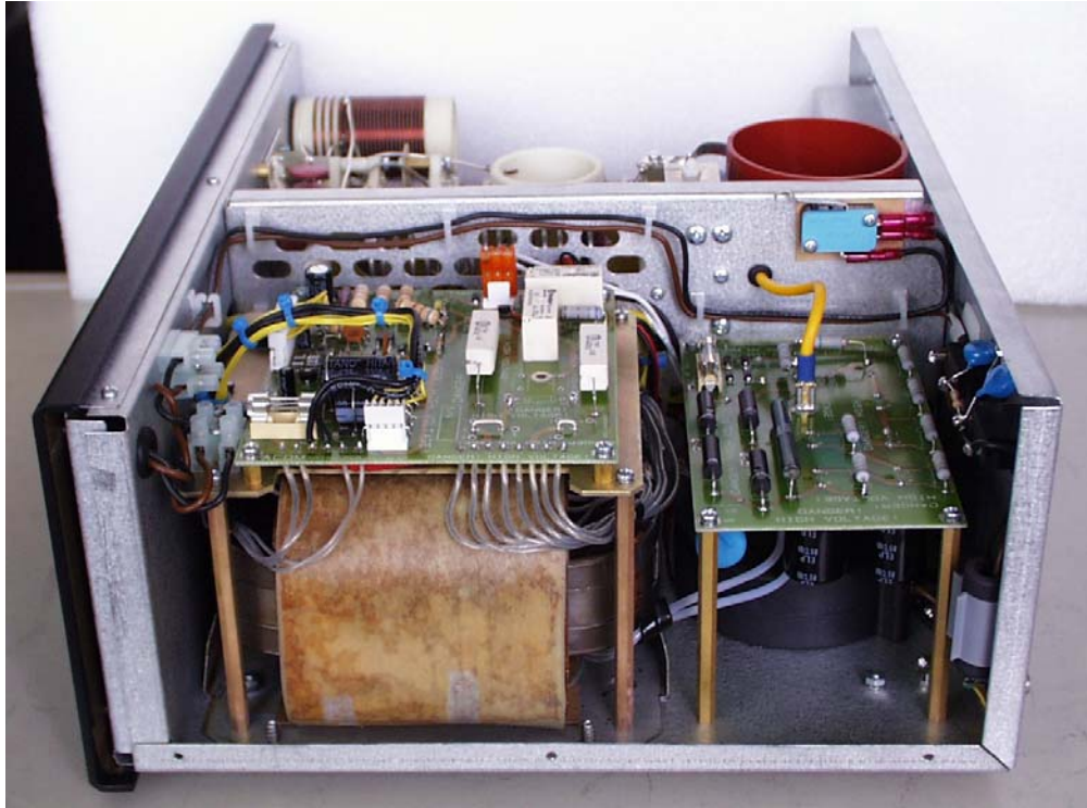
Fig.1 Right side View
