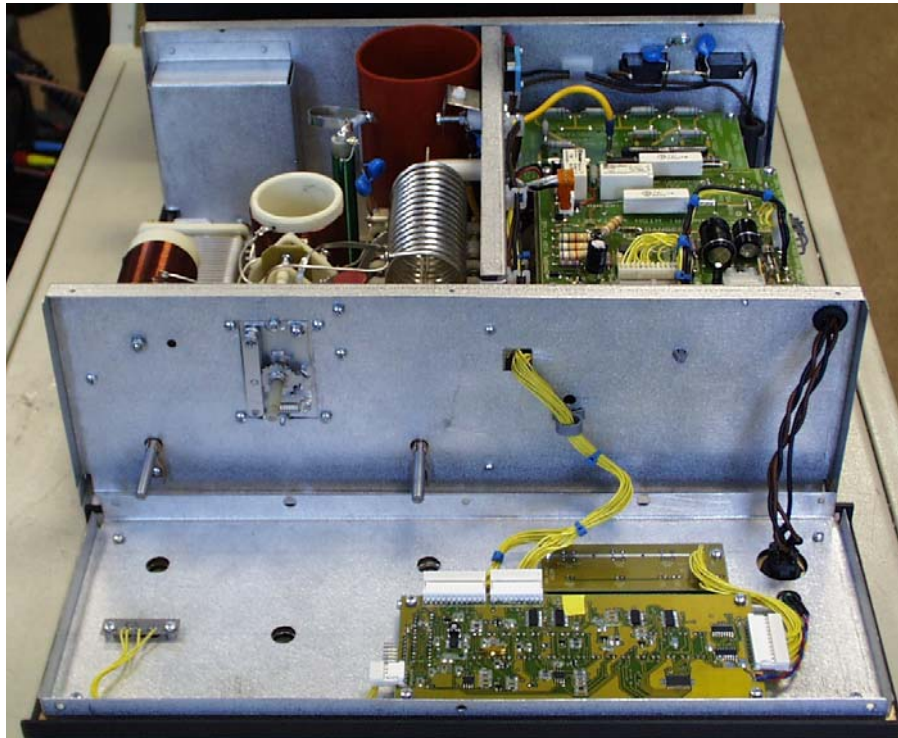
Fig.3 Front panel lay down
