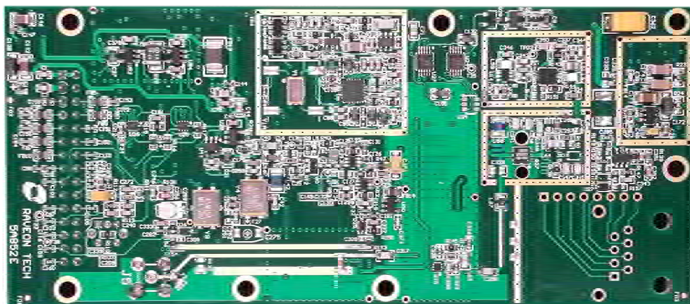
PCB RF Board - Top
