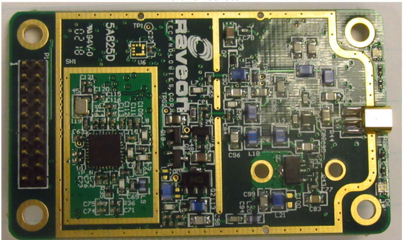
Front with no Shields
