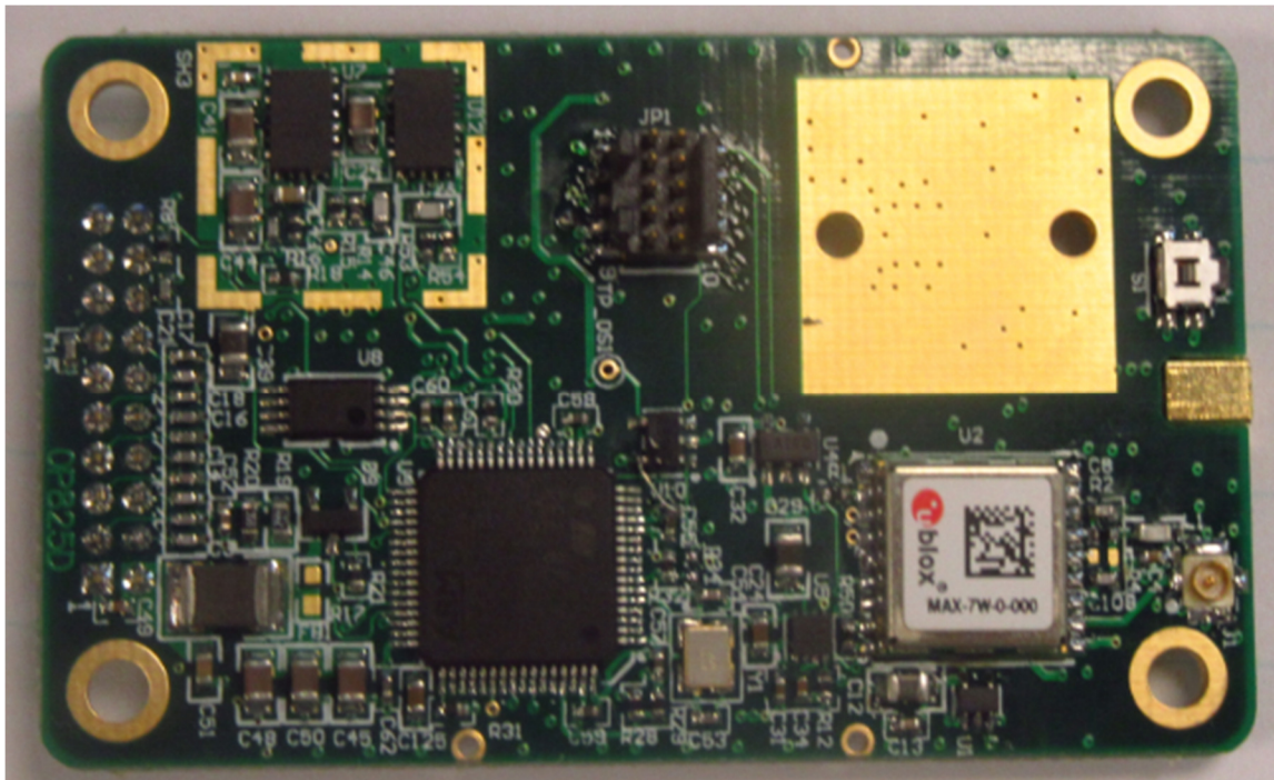
Back with no Shields
