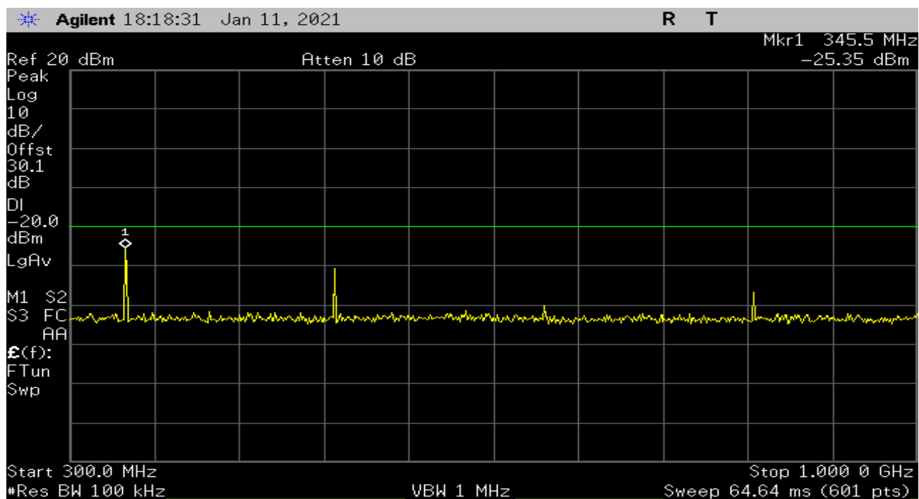
Plot 23 – High Band
