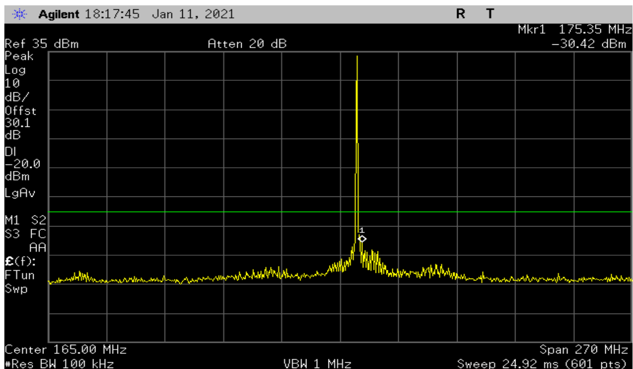
Plot 22 – High Band
