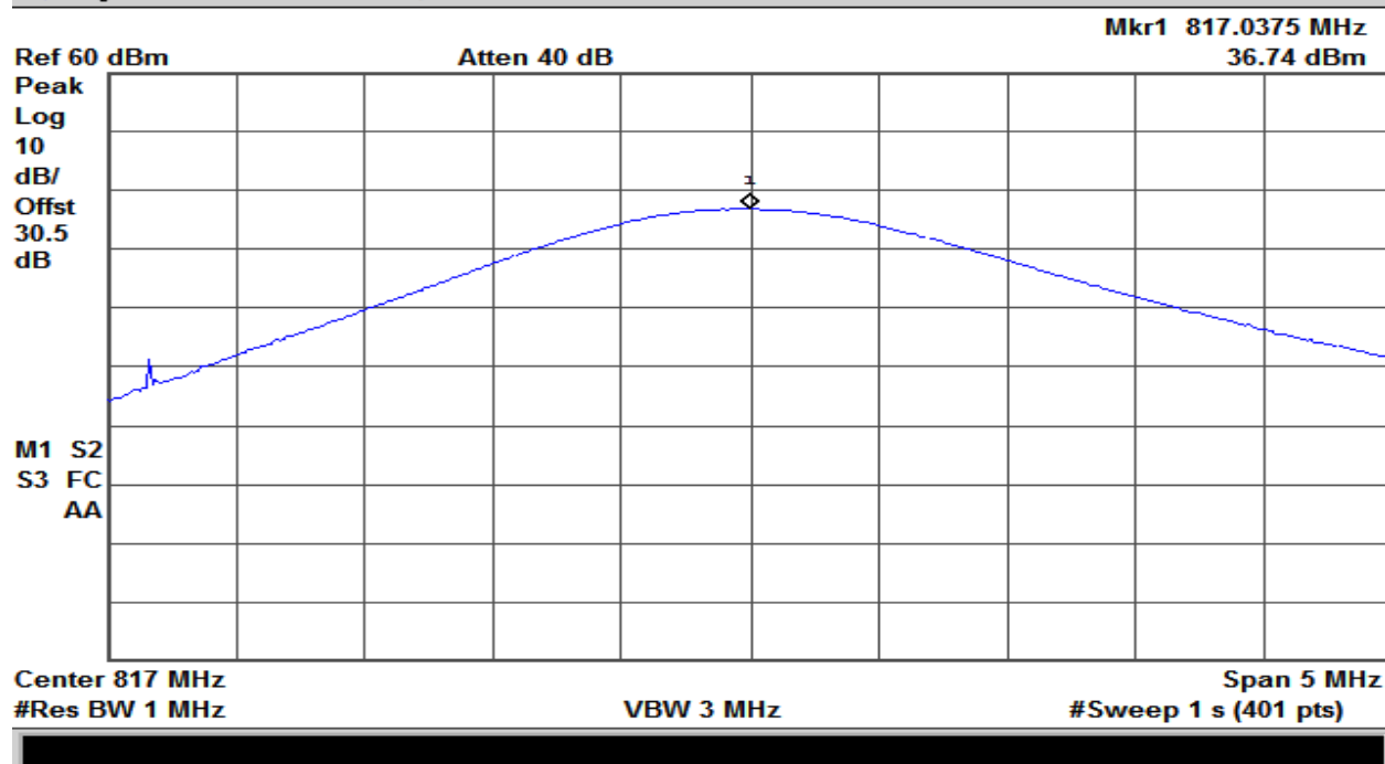
Plot 3 – Output Power – High
