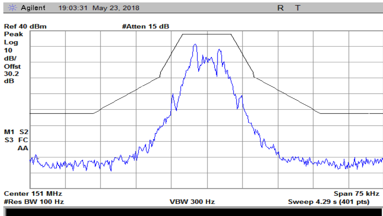
Plot 9 – Low Channel at Wideband Band 25 kHz Spacing – Mask C
