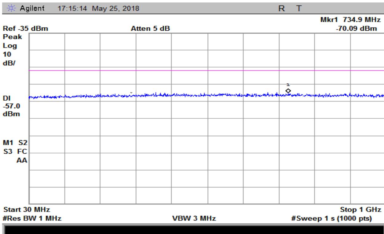
Plot 21 – Receiver Emission – For Industry Canada Only (RSS-GEN)
