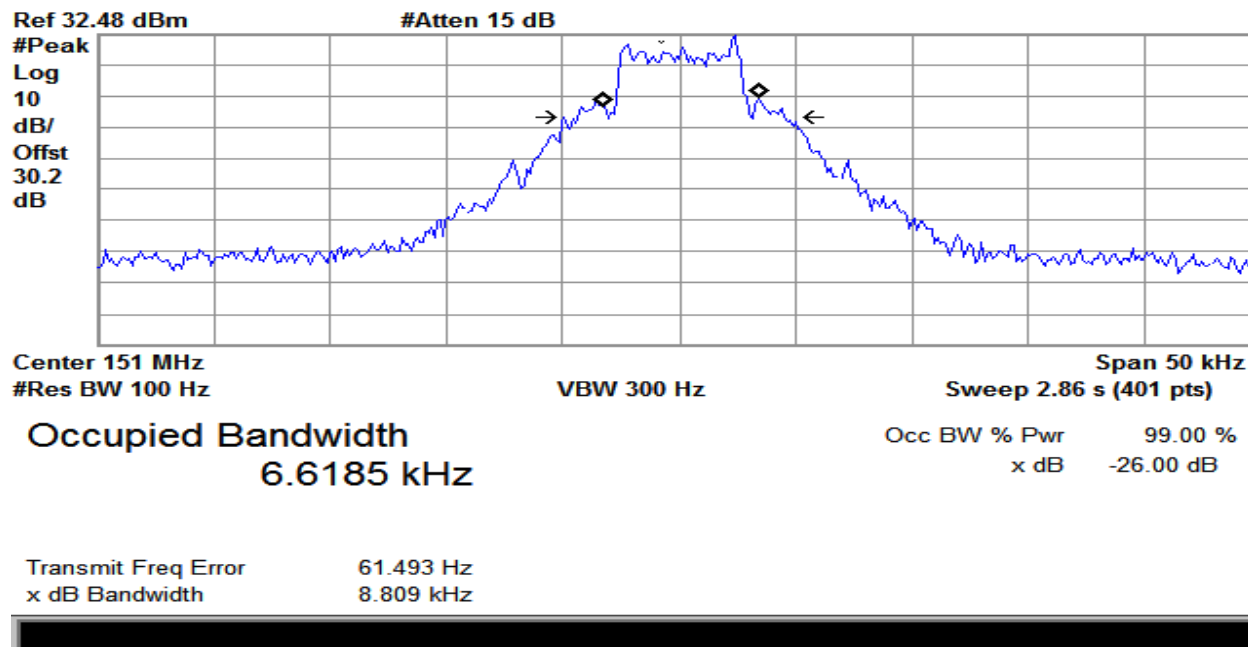
Plot 4 – Narrow Band
