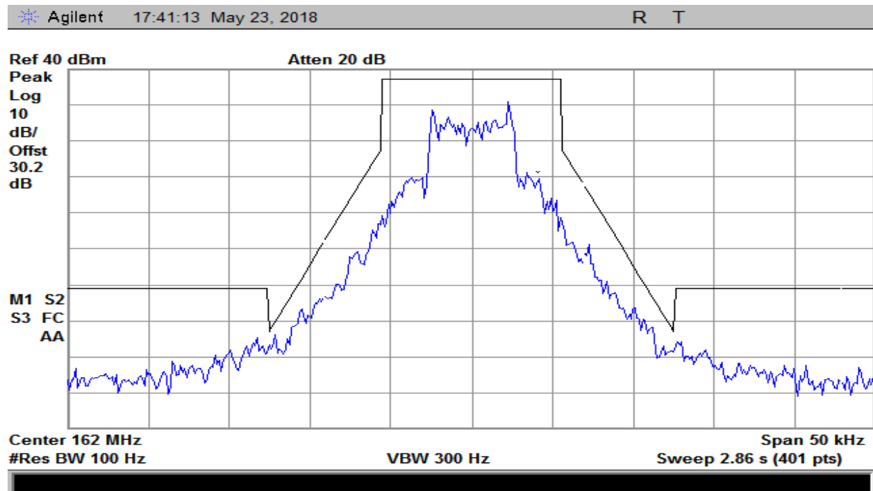
Plot 7 – Mid Channel at Narrow Band 12.5 kHz Spacing – Mask D
