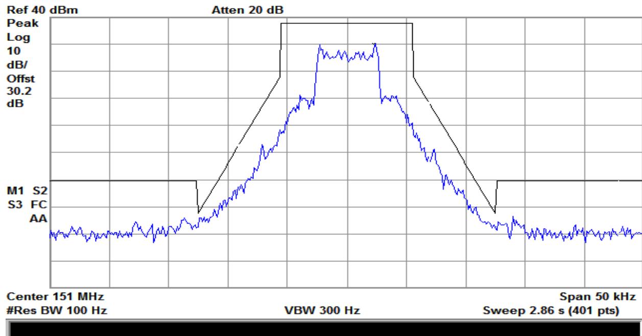
Plot 6 – Low Channel at Narrow Band 12.5 kHz Spacing – Mask D
