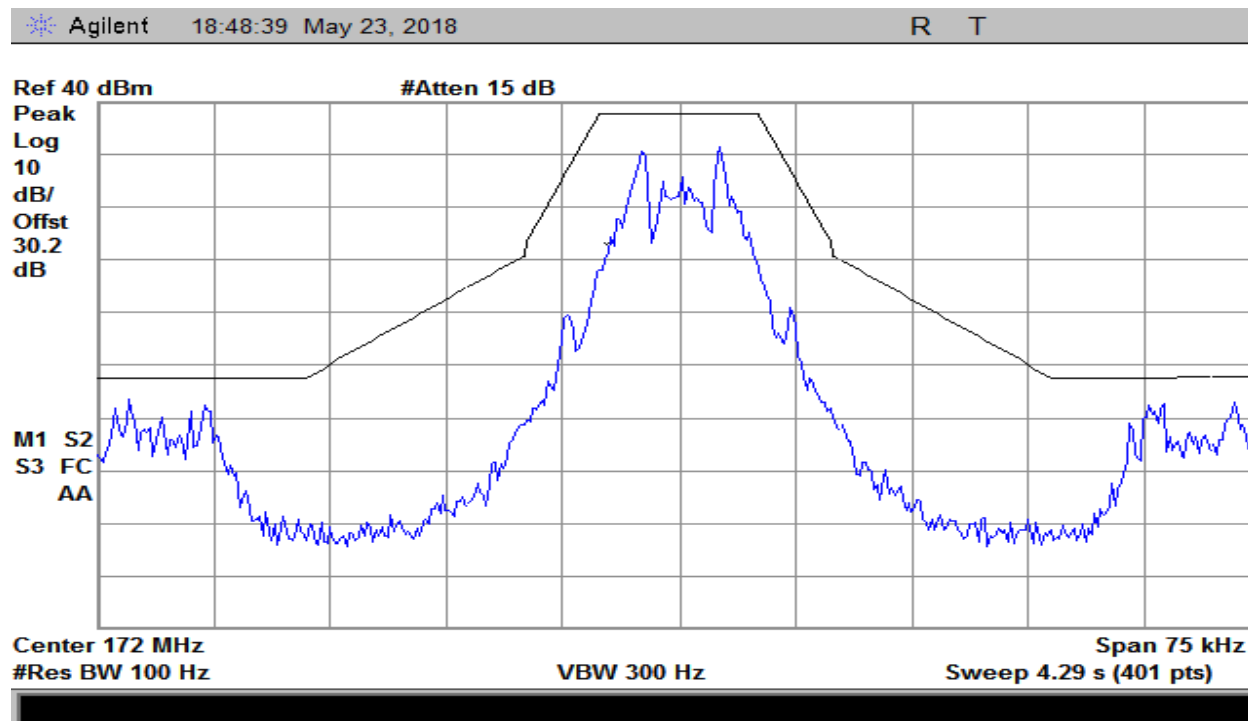
Plot 11 – High Chanel at Wideband Band 25 kHz Spacing – Mask C
