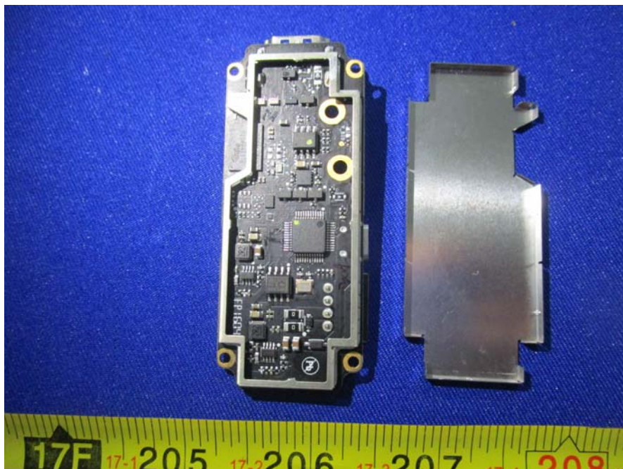
EUT- Unshield View
