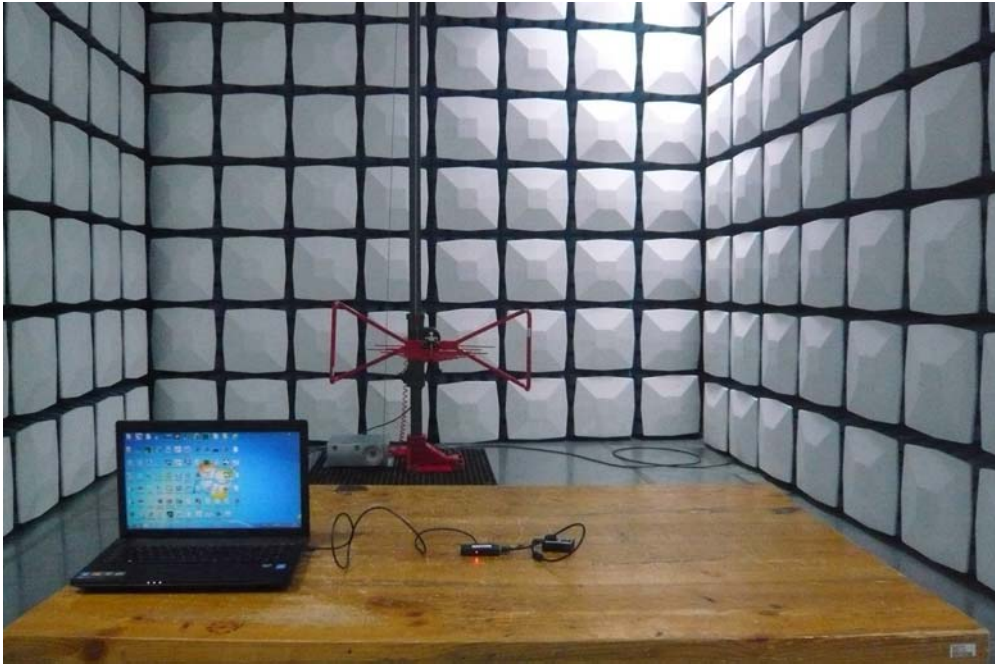
Radiated Emission View (Below 1GHz)-Battery Mode
