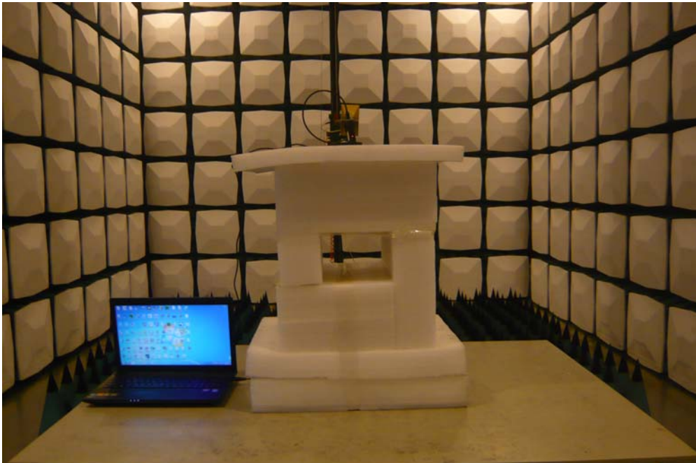
Radiated Emission View (Above 1GHz) -Battery Mode
