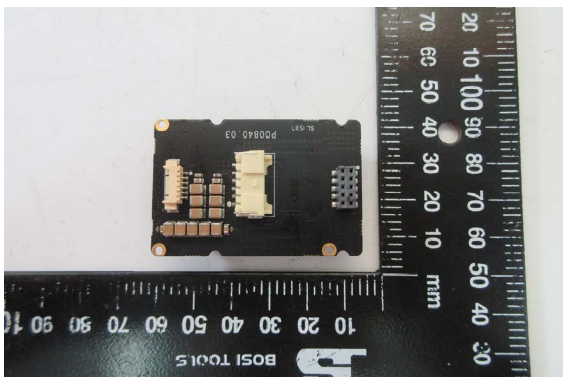
4. Sub board front view
