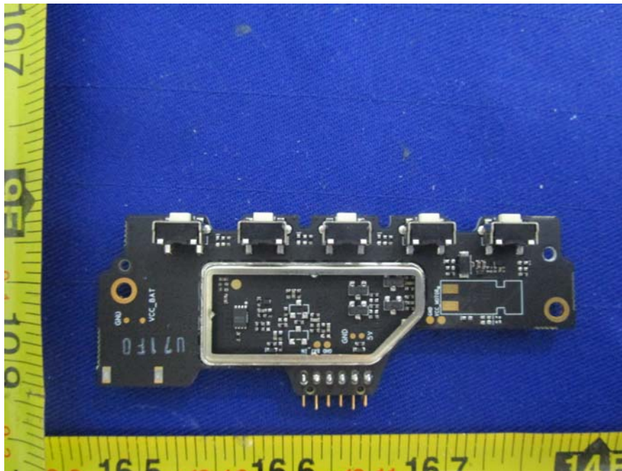
EUT –Board Bottom Unshielded View
