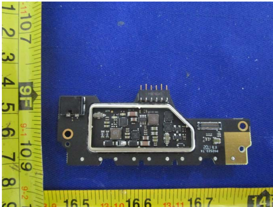
EUT – Board Top Unshielded View
