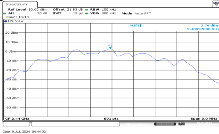
BLE_2M_Ant5_2440_0~Reference
