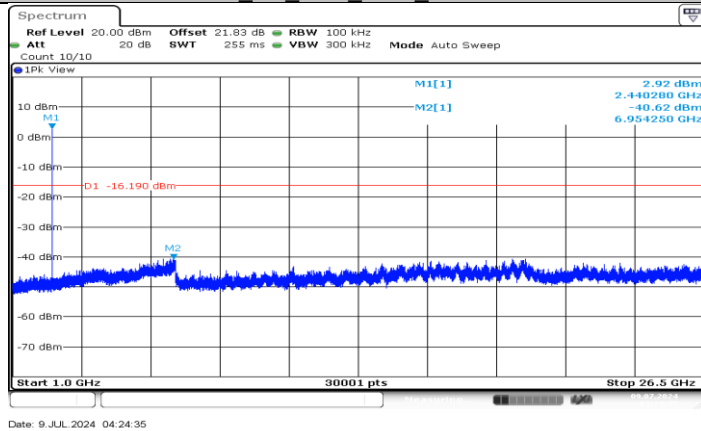
BLE_1M_Ant5_2440_1000~26500
