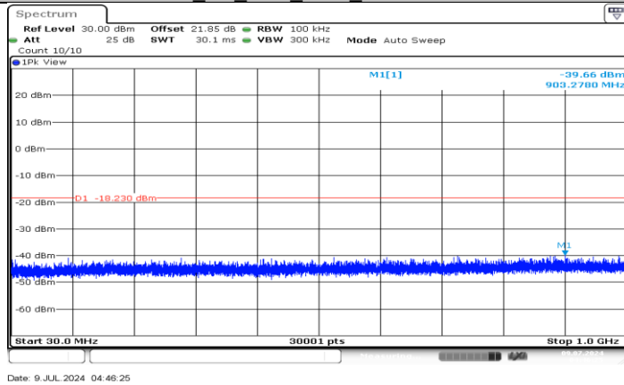
BLE_2M_Ant5_2480_30~1000
