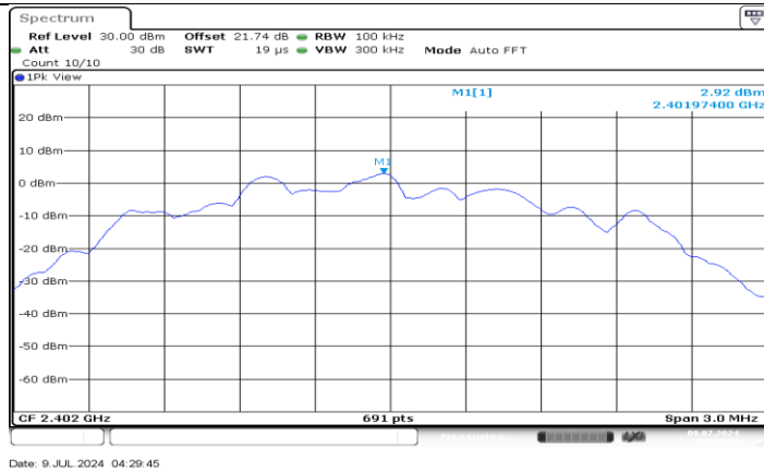
BLE_2M_Ant5_2402_0~Reference
