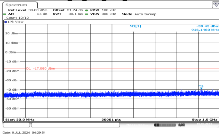
BLE_2M_Ant5_2402_30~1000
