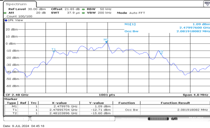
BLE_2M_Ant5_2480
