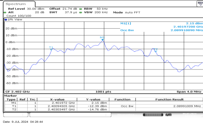
BLE_2M_Ant5_2402
