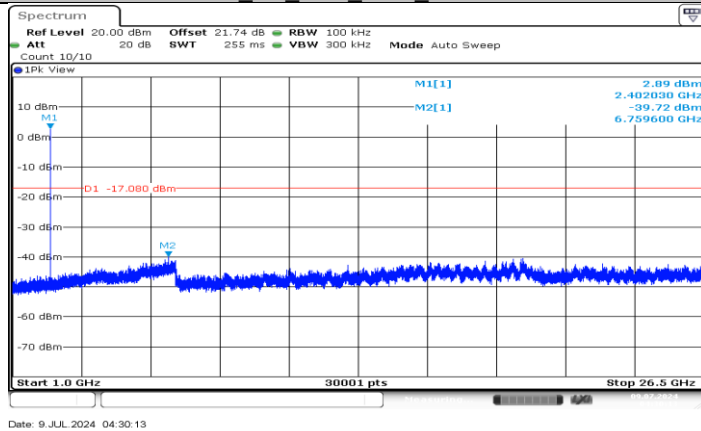
BLE_2M_Ant5_2402_1000~26500
