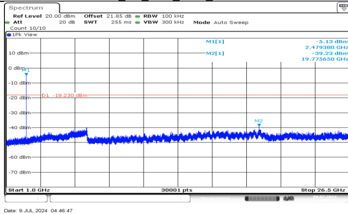
BLE_2M_Ant5_2480_1000~26500
