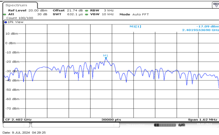
BLE_2M_Ant5_2402
