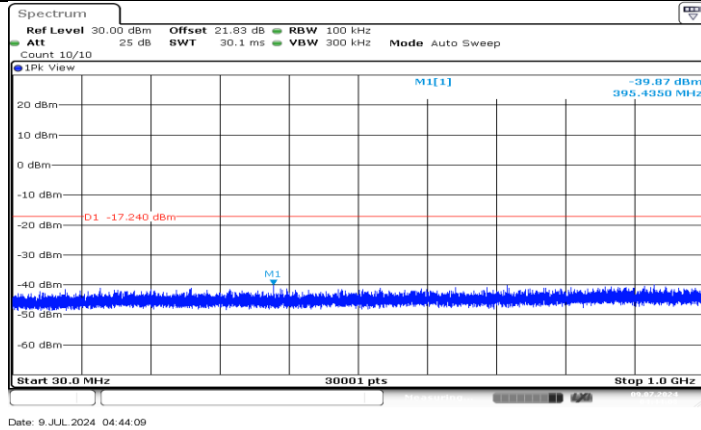
BLE_2M_Ant5_2440_30~1000
