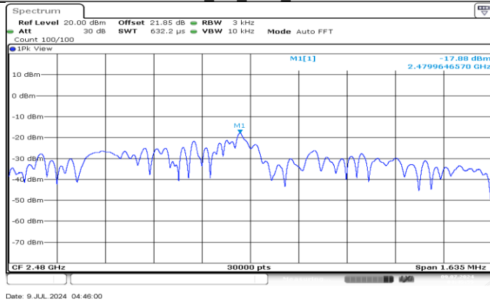
BLE_2M_Ant5_2480
