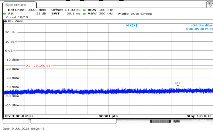
BLE_1M_Ant5_2440_30~1000
