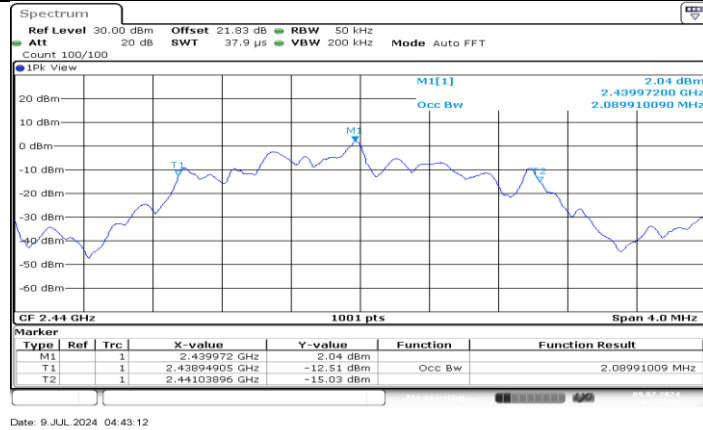
BLE_2M_Ant5_2440
