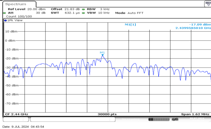
BLE_2M_Ant5_2440
