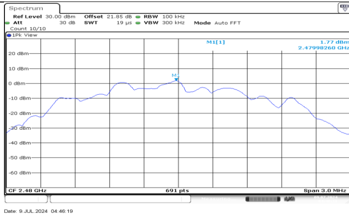
BLE_2M_Ant5_2480_0~Reference
