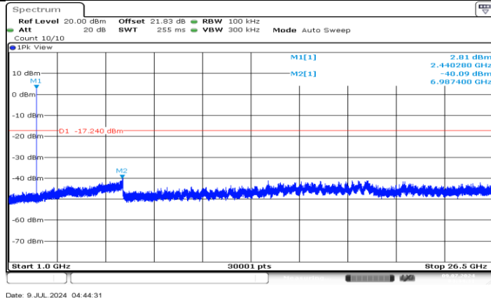
BLE_2M_Ant5_2440_1000~26500
