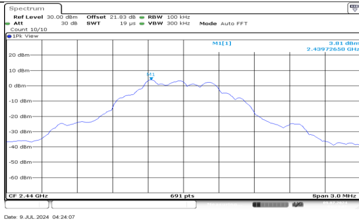
BLE_1M_Ant5_2440_0~Reference
