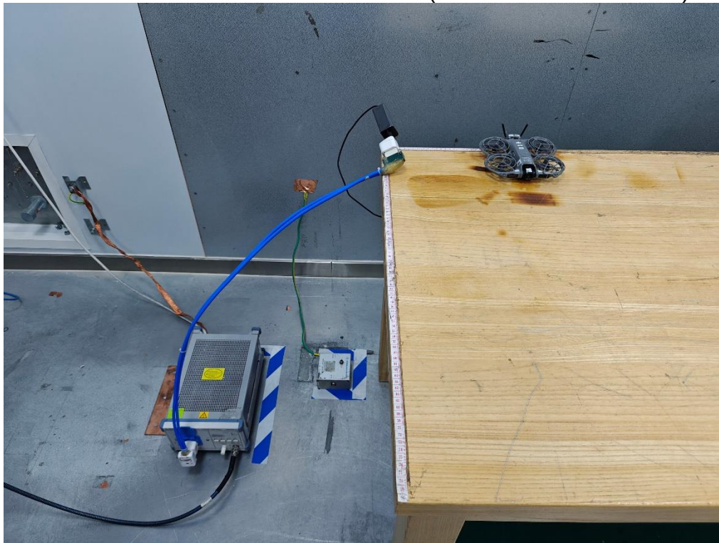
RADIATED RF MEASUREMENT SETUP (AC Conducted Power Line)
