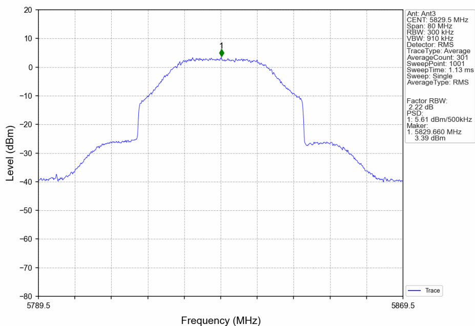
40M_HCH_5829.5MHz_Ant3_NTNV
