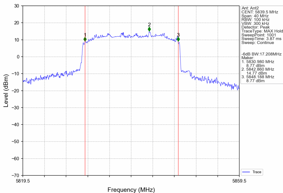
20M_HCH_5839.5MHz_Ant2_NTNV
