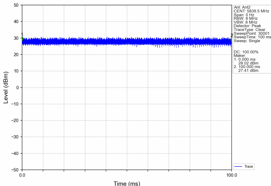
20M_HCH_5839.5MHz_Ant2_NTNV
