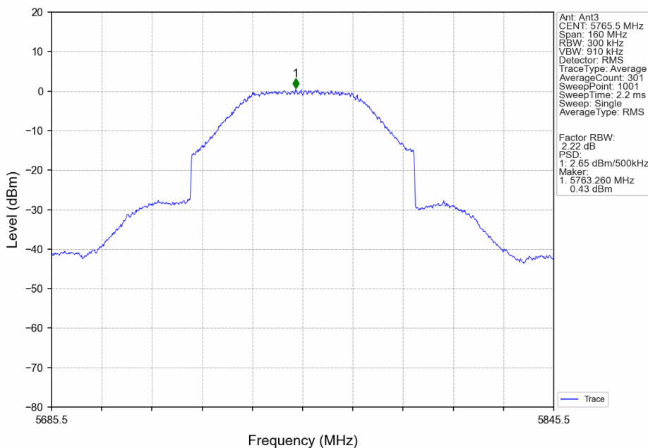
80M_LCH_5765.5MHz_Ant3_NTNV
