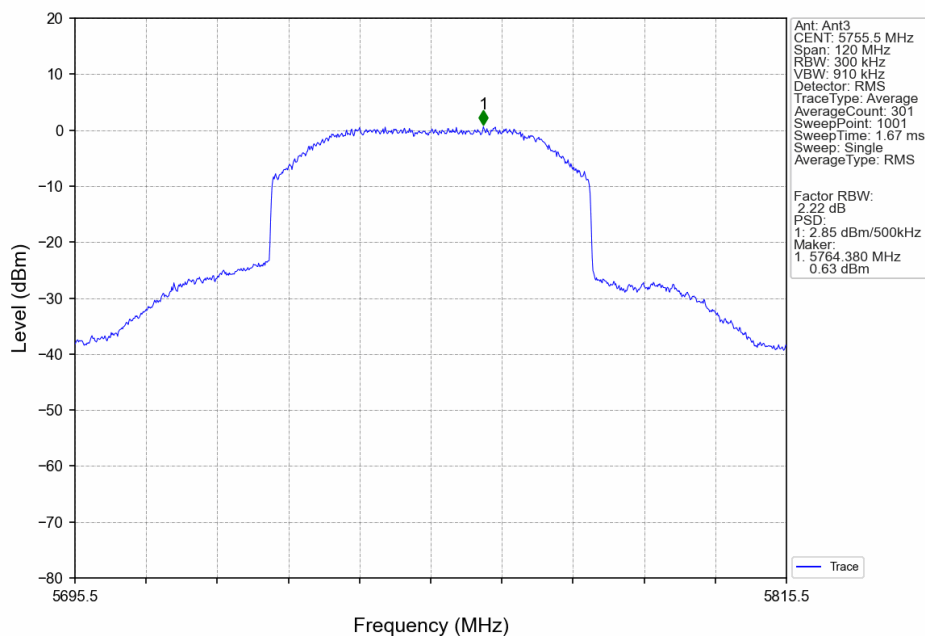
60M_LCH_5755.5MHz_MIMO_NTNV
