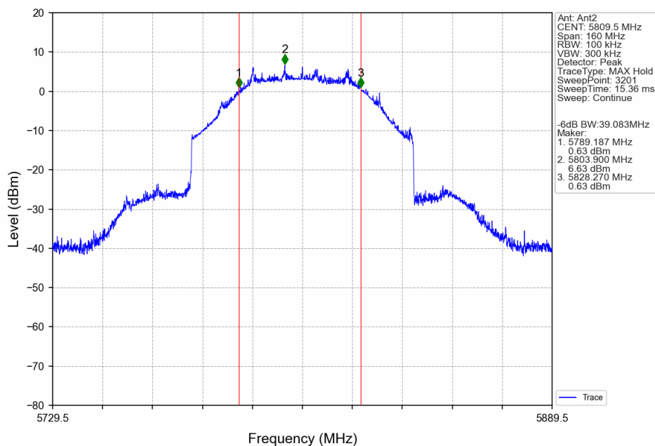
80M_HCH_5809.5MHz_Ant2_NTNV
