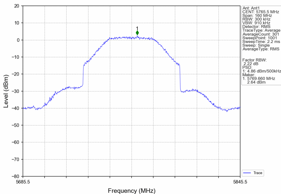
80M_LCH_5765.5MHz_Ant1_NTNV
