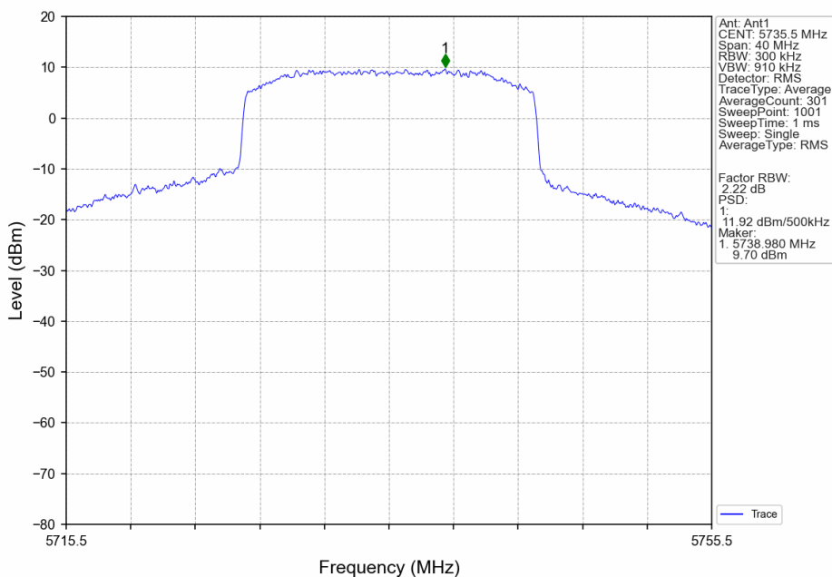
20M_LCH_5735.5MHz_MIMO_NTNV
