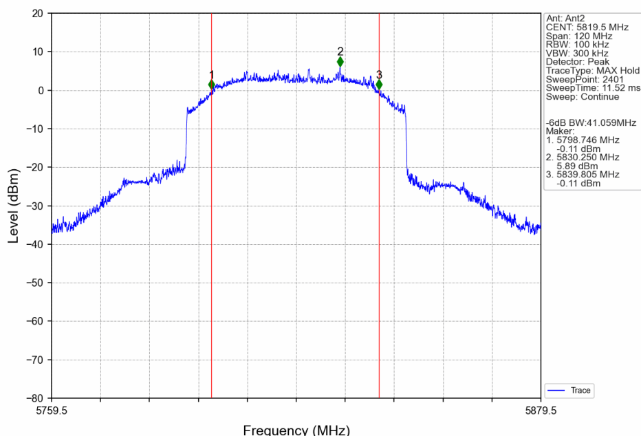
60M_HCH_5819.5MHz_Ant2_NTNV
