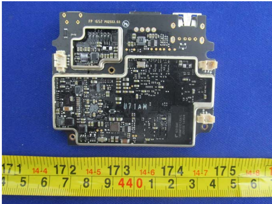
EUT – Board 1 Bottom Unshielded View
