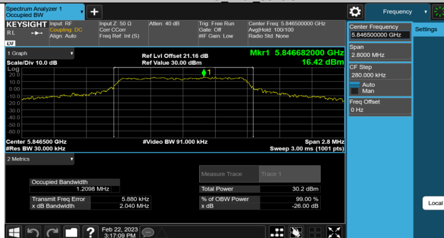
1.4M-MIMO Ant1 5846.5
