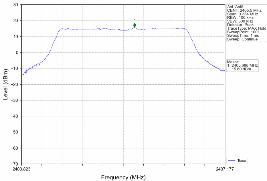
3M_LCH_2405.5MHz_Ant5_NTNV
