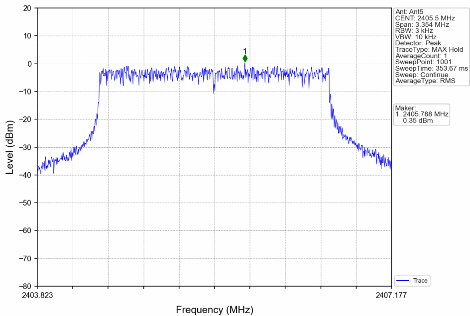
3M_LCH_2405.5MHz_Ant5_NTNV
