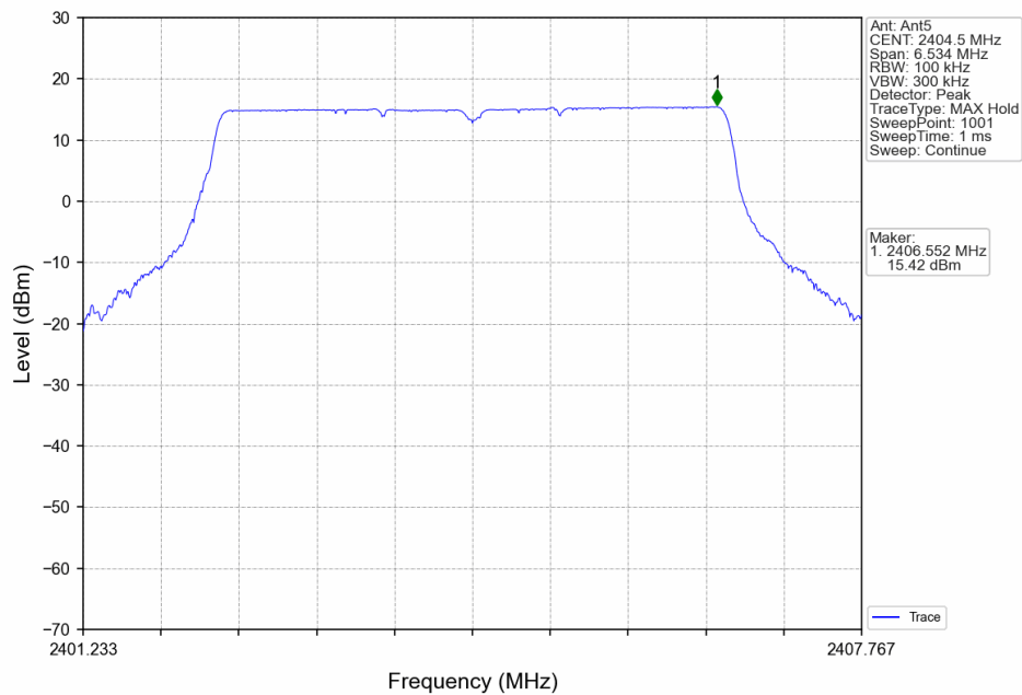
5M_LCH_2404.5MHz_Ant5_NTNV
