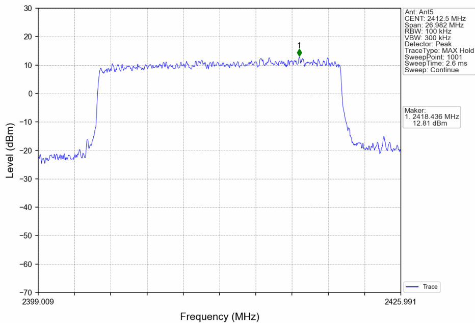
20M_LCH_2412.5MHz_Ant5_NTNV
