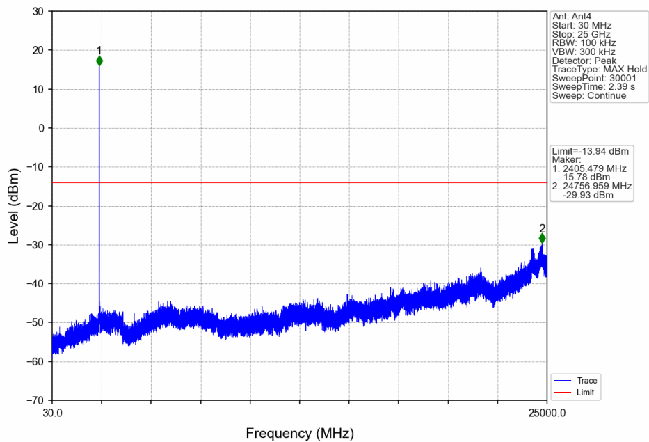
3M_LCH_2405.5MHz_Ant4_NTNV
