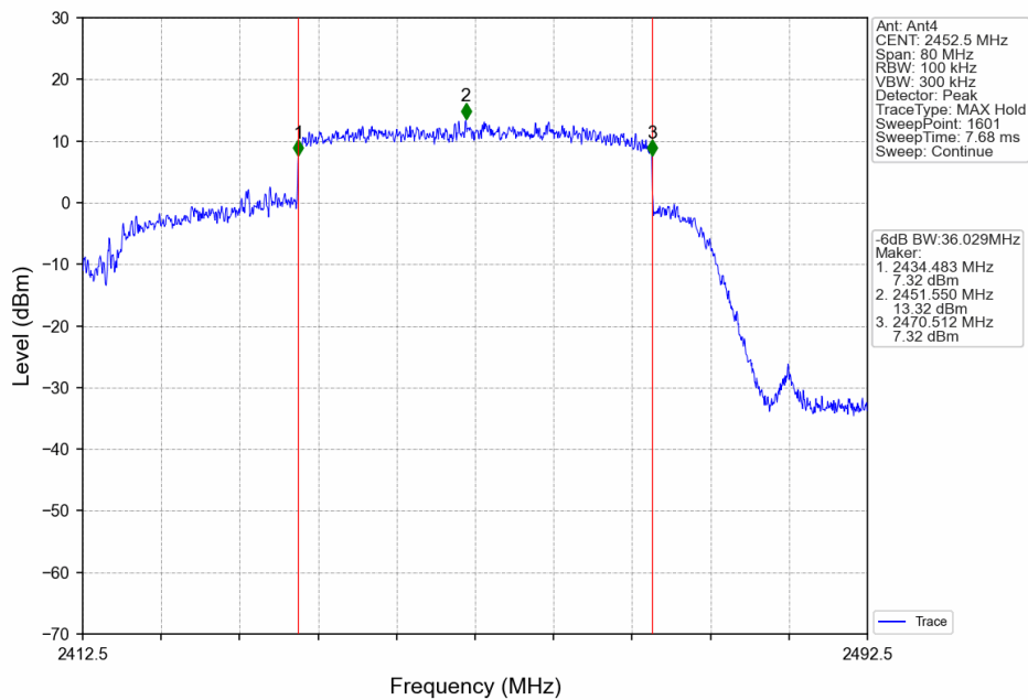
40M_HCH_2452.5MHz_Ant4_NTNV
