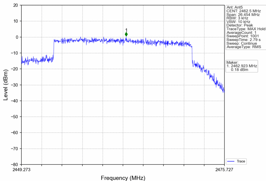
20M_HCH_2462.5MHz_Ant5_NTNV
