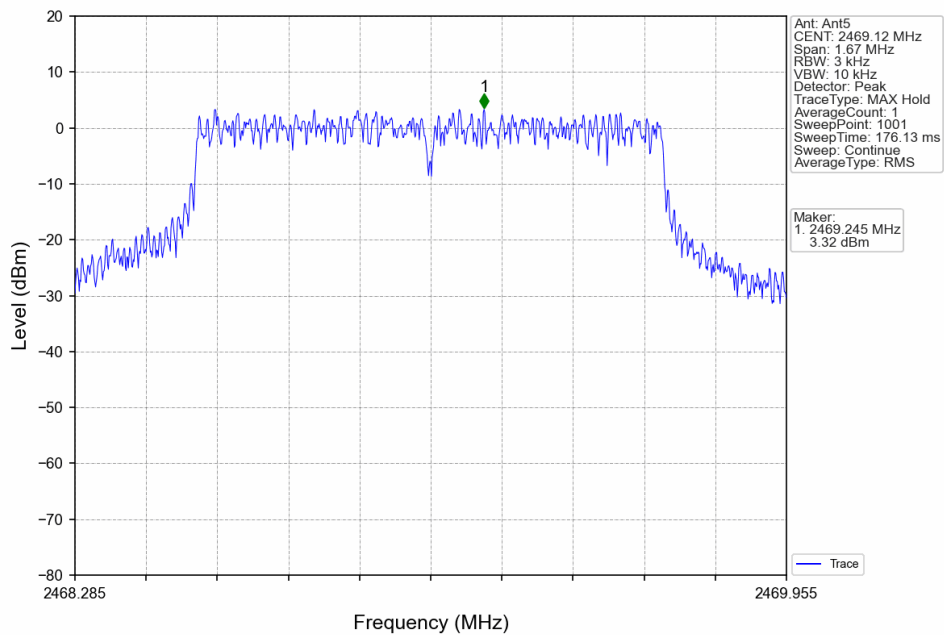
1.4M_HCH_2469.12MHz_Ant5_NTNV
