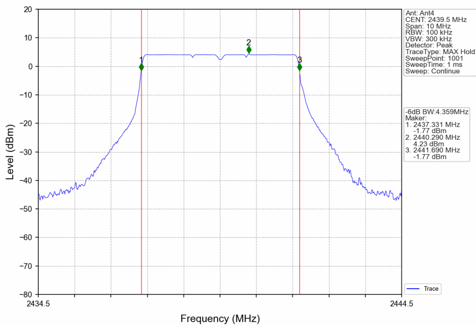
5M_MCH_2439.5MHz_Ant4_NTNV
