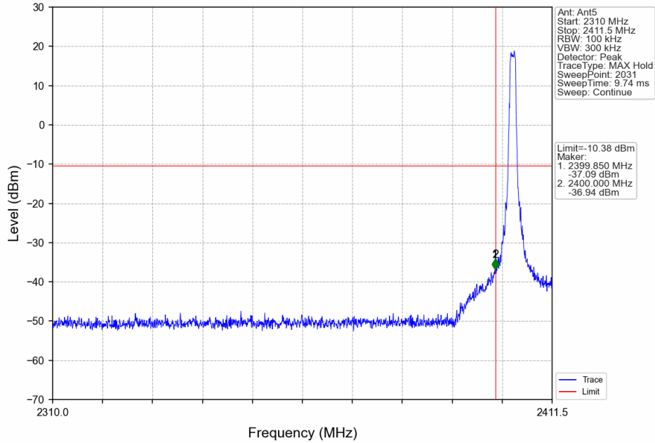
1.4M_LCH_2403.5MHz_Ant5_NTNV
