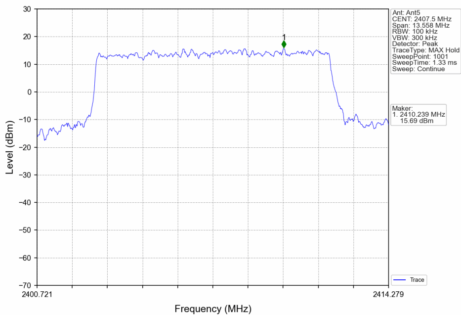
10M_LCH_2407.5MHz_Ant5_NTNV
