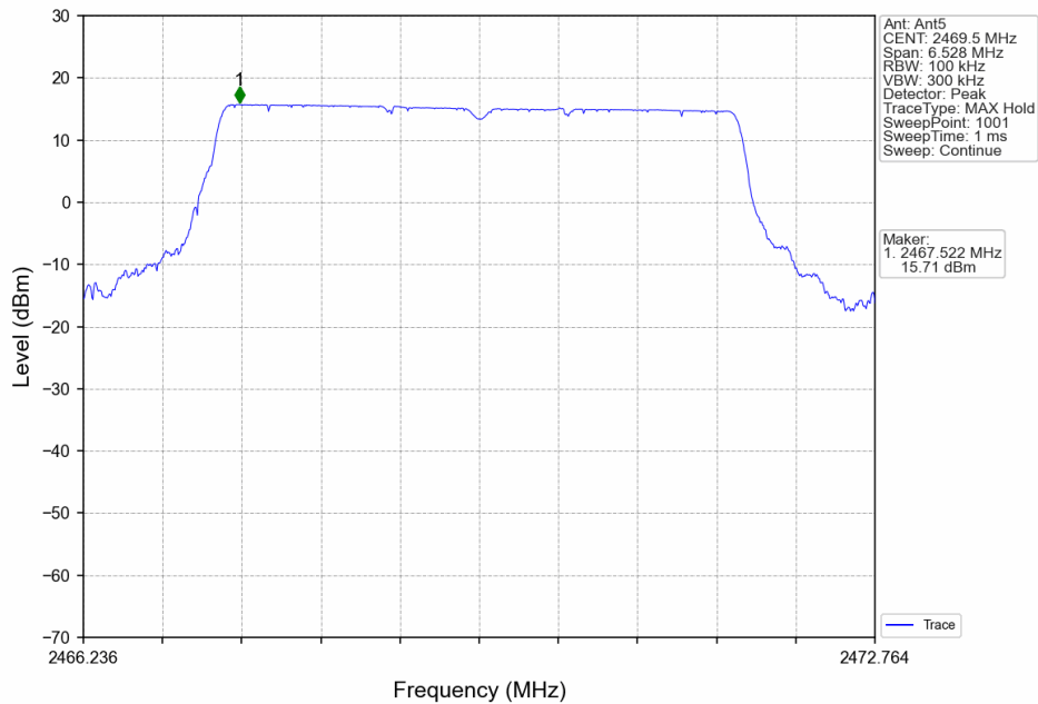
5M_HCH_2469.5MHz_Ant5_NTNV
