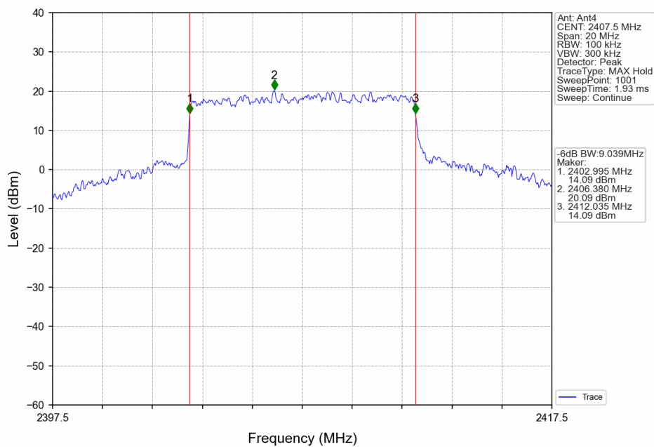
10M_LCH_2407.5MHz_Ant4_NTNV
