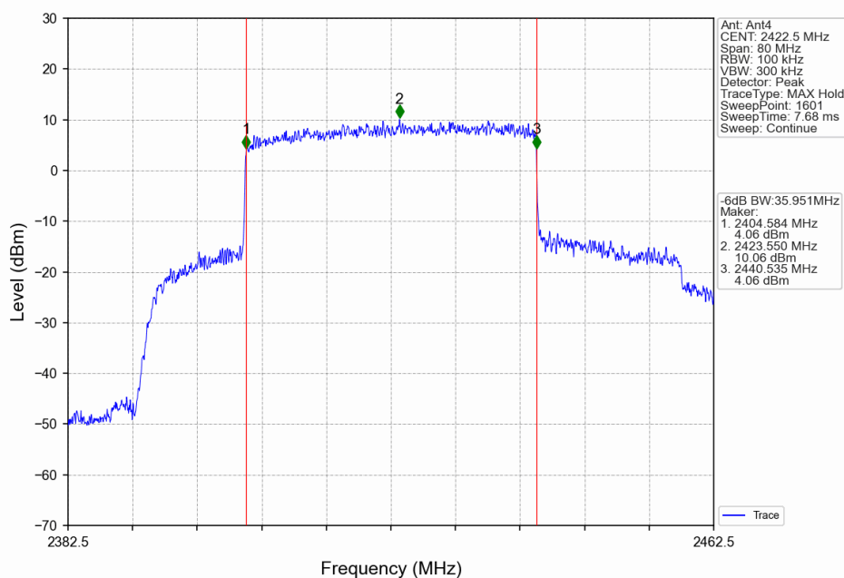
40M_LCH_2422.5MHz_Ant4_NTNV
