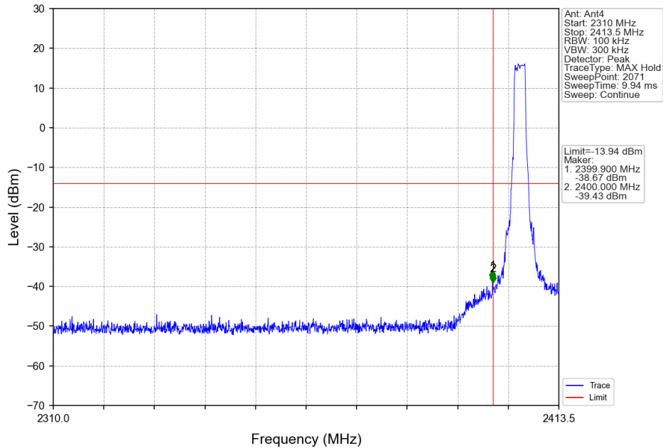
3M_LCH_2405.5MHz_Ant4_NTNV
