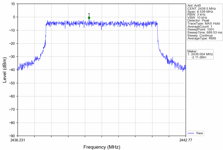
5M_MCH_2439.5MHz_Ant5_NTNV
