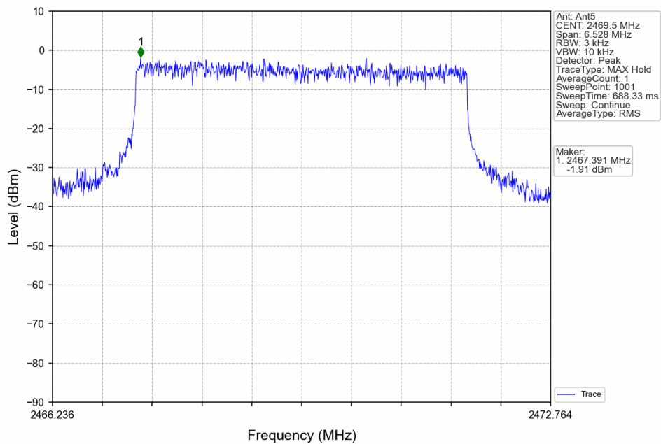
5M_HCH_2469.5MHz_Ant5_NTNV
