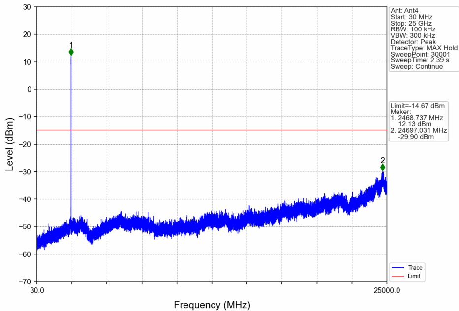
5M_HCH_2469.5MHz_Ant4_NTNV
