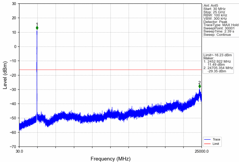
40M_HCH_2452.5MHz_Ant5_NTNV
