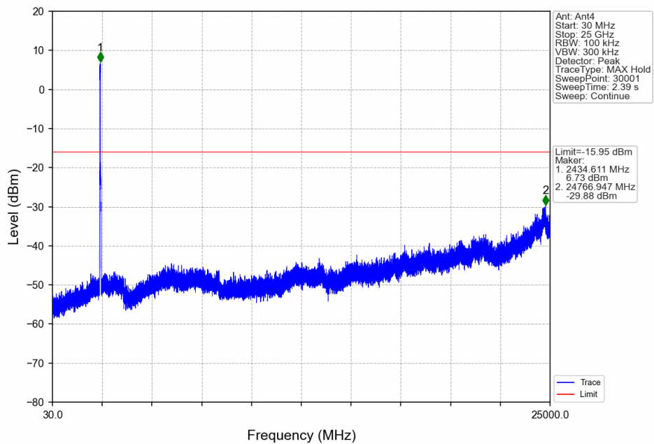
40M_LCH_2422.5MHz_Ant4_NTNV
