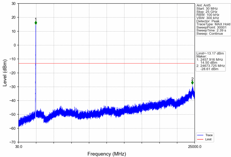
20M_HCH_2462.5MHz_Ant5_NTNV
