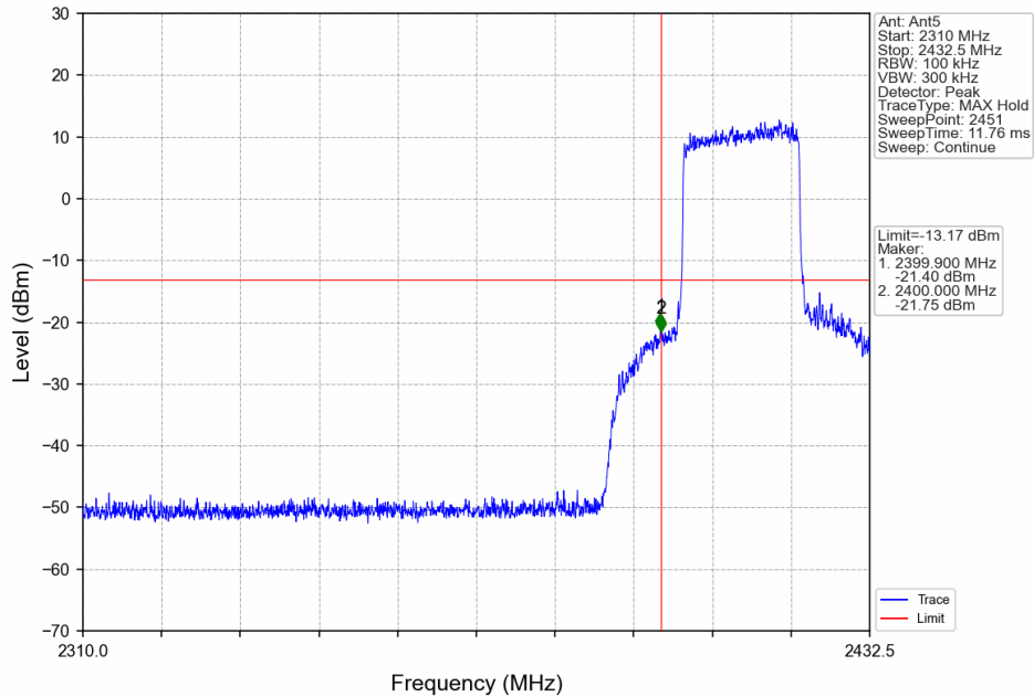
20M_LCH_2412.5MHz_Ant5_NTNV
