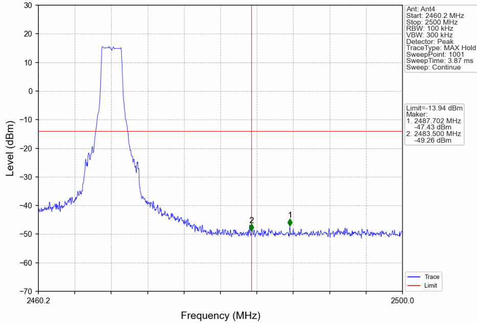
3M_HCH_2468.2MHz_Ant4_NTNV
