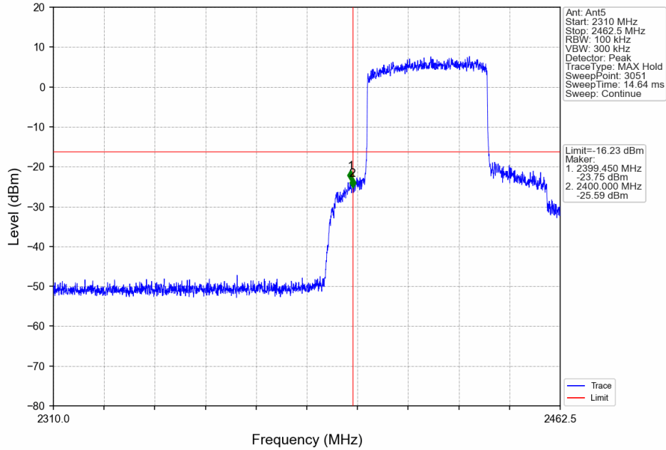
40M_LCH_2422.5MHz_Ant5_NTNV
