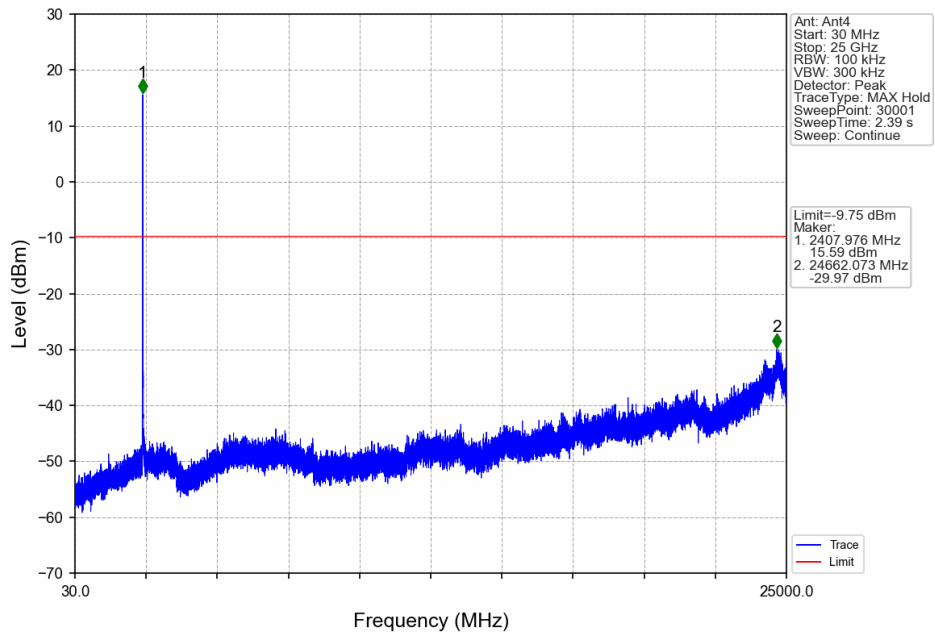
10M_LCH_2407.5MHz_Ant4_NTNV
