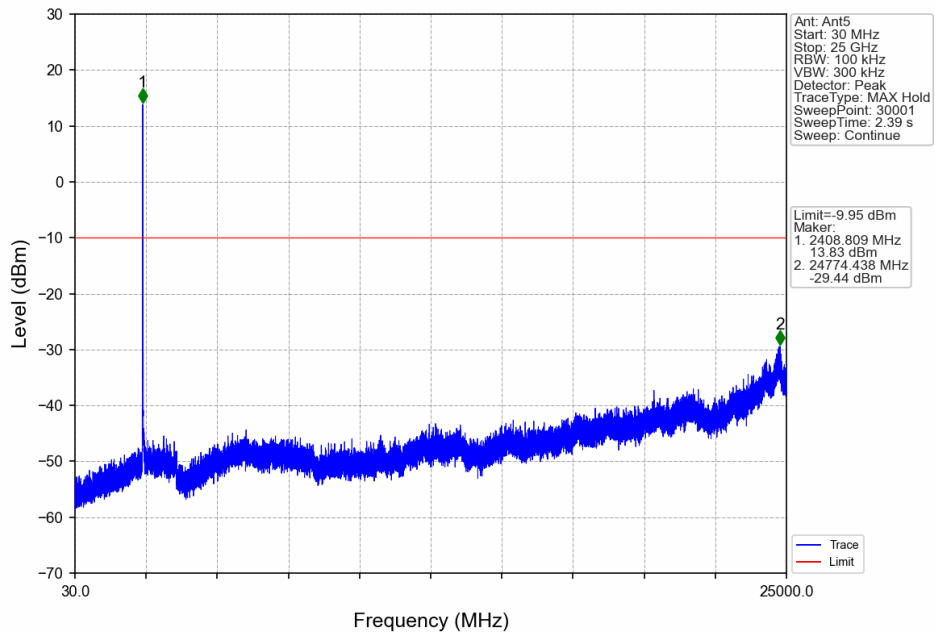
10M_LCH_2407.5MHz_Ant5_NTNV
