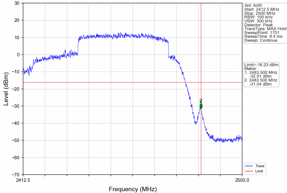
40M_HCH_2452.5MHz_Ant5_NTNV
