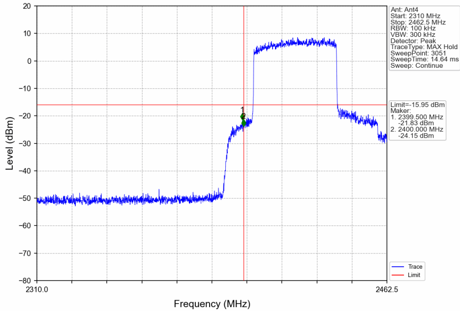
40M_LCH_2422.5MHz_Ant4_NTNV
