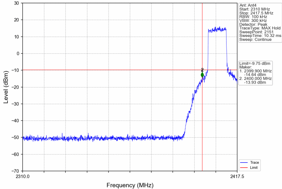
10M_LCH_2407.5MHz_Ant4_NTNV
