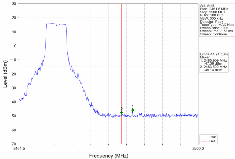
5M_HCH_2469.5MHz_Ant5_NTNV
