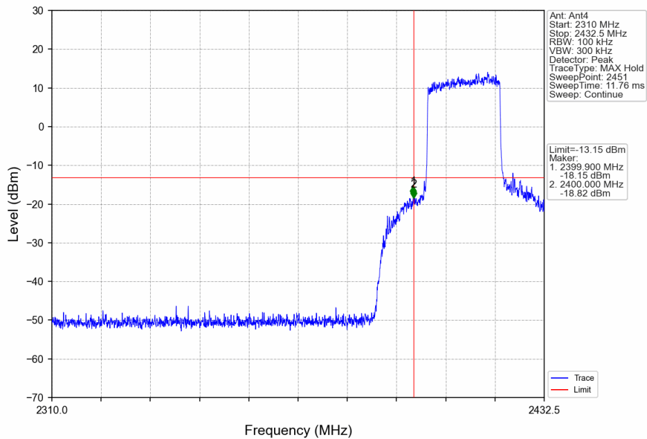
20M_LCH_2412.5MHz_Ant4_NTNV
