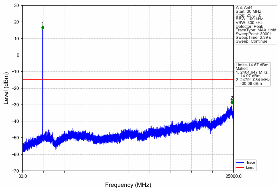
5M_LCH_2404.5MHz_Ant4_NTNV
