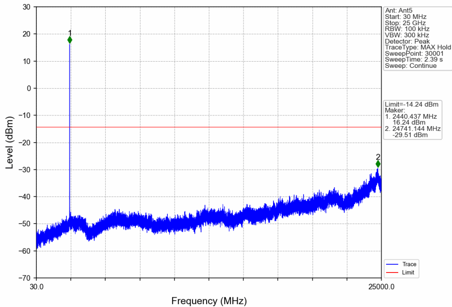
5M_MCH_2439.5MHz_Ant5_NTNV
