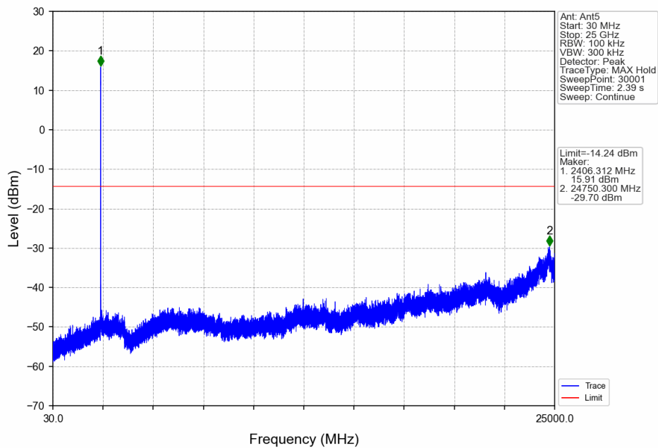
5M_LCH_2404.5MHz_Ant5_NTNV
