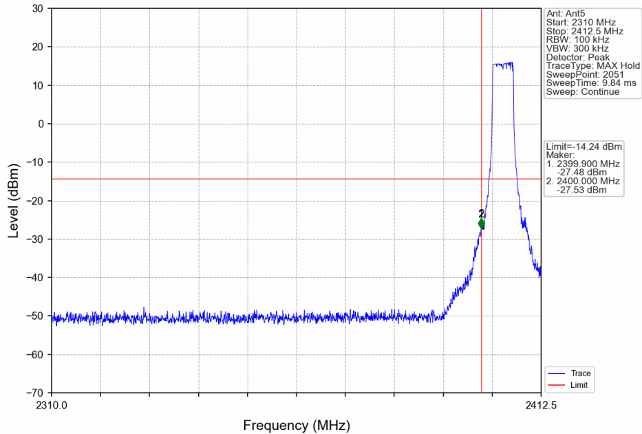
5M_LCH_2404.5MHz_Ant5_NTNV
