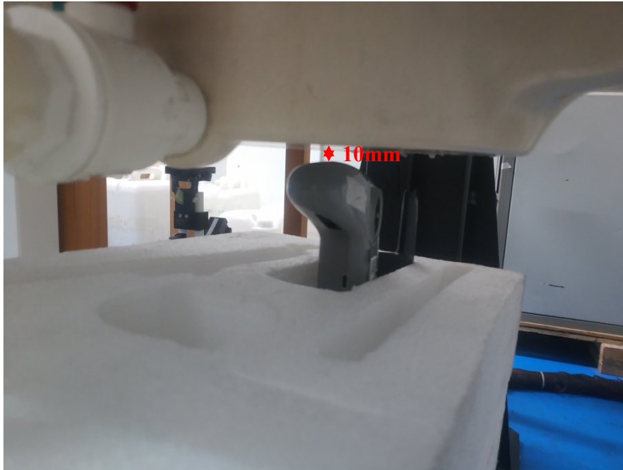
Close to Body Left Setup Photo (10mm)
