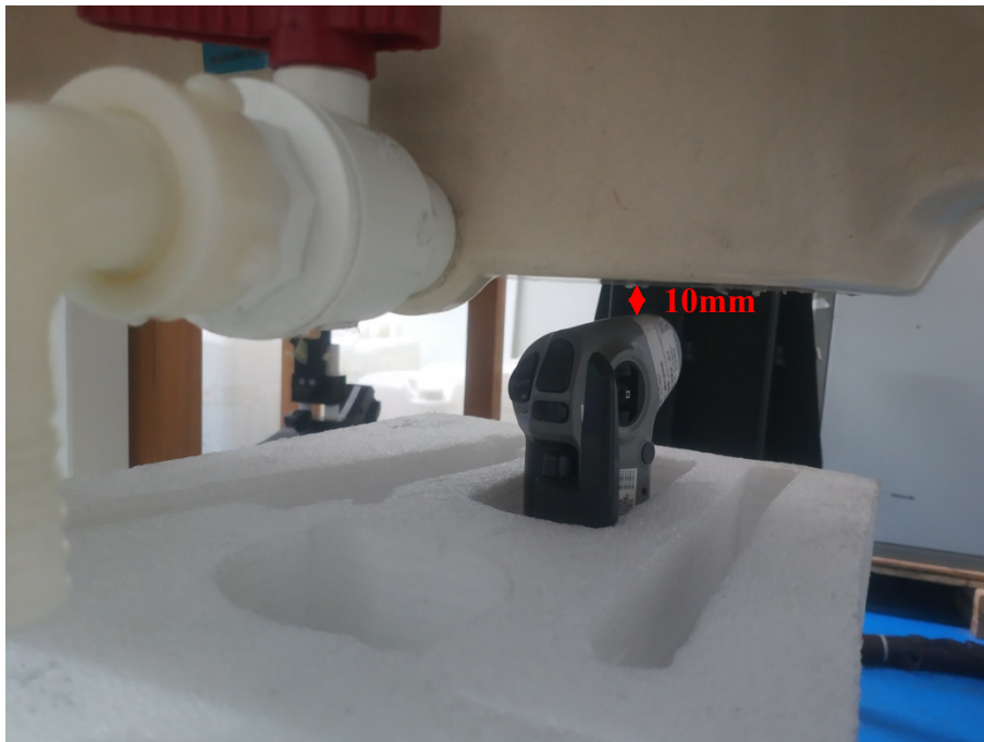
Close to Body Right Setup Photo (10mm)
