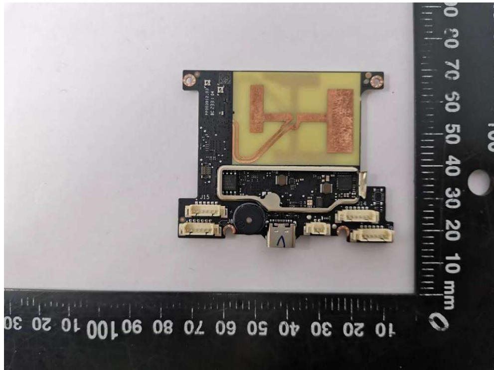
Fig.6. PCB view 1
