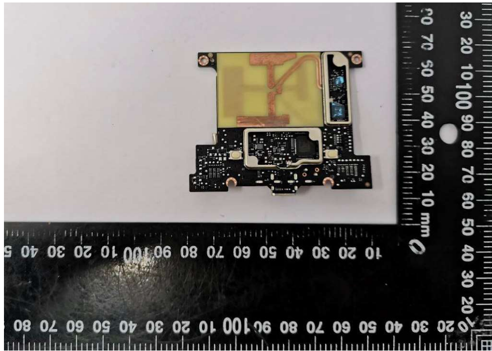
Fig.7. PCB view 2
