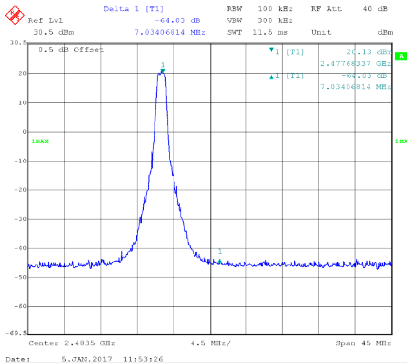
Chain 0-1.4M Band Edge, Right Side
