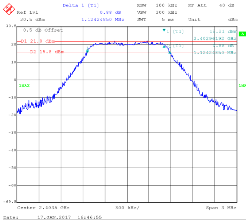
1.4M Low Channel
