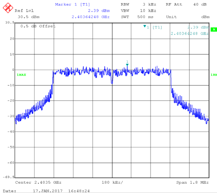
Chain 0-Power Spectral Density,1.4M Low Channel
