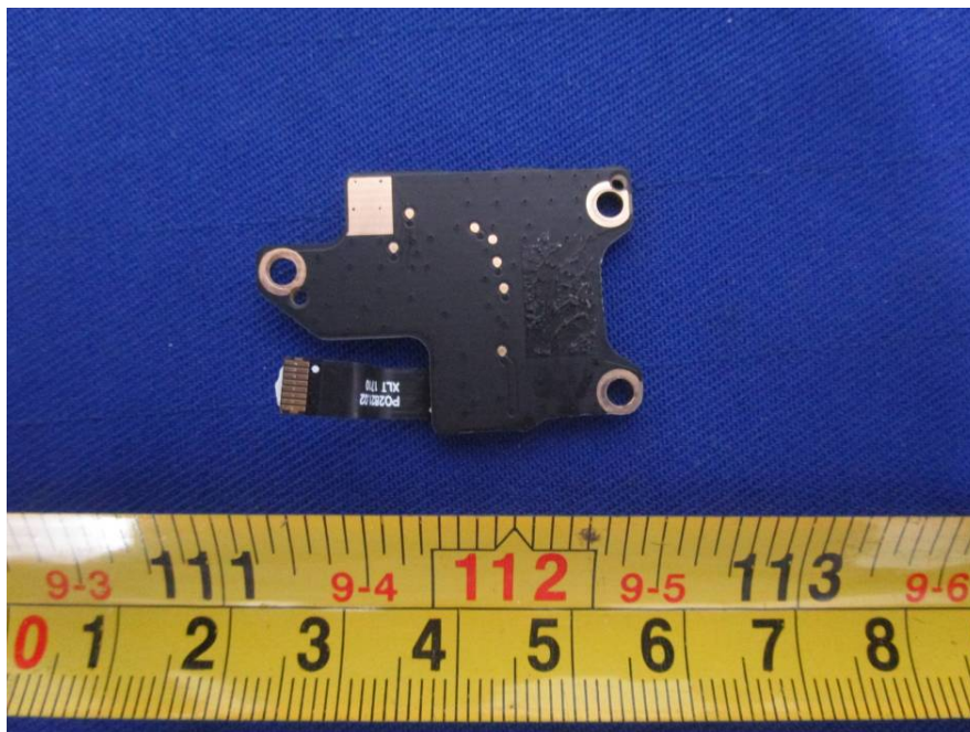
EUT –Left Subboard Bottom View
