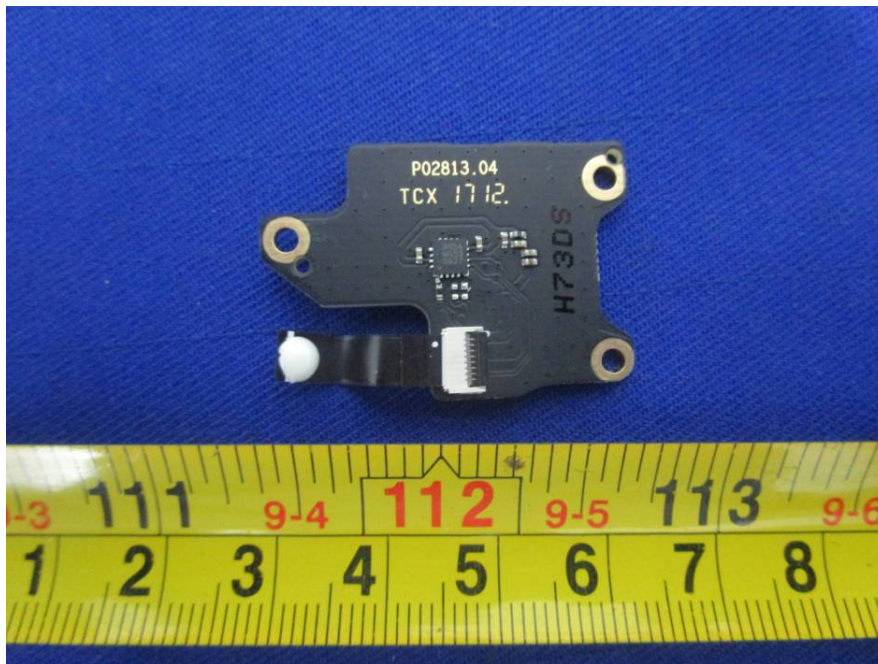
EUT –Right Subboard Top View
