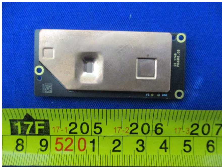
EUT –SDR Module Board Top View
