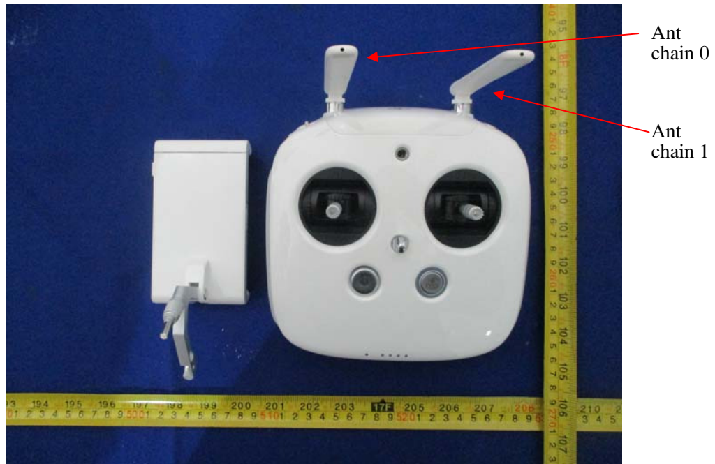
EUT – Uncover-1 View
