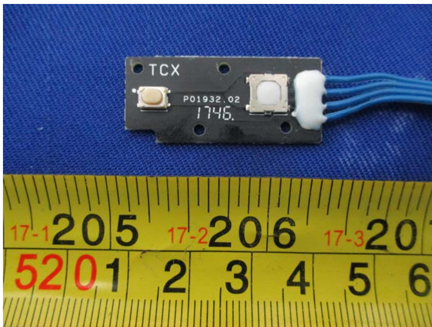
EUT – PCB-10 Top View
