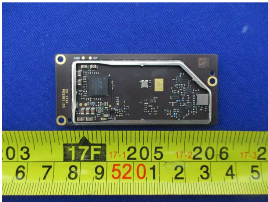
EUT – SDR Module Board Top Uncover View
