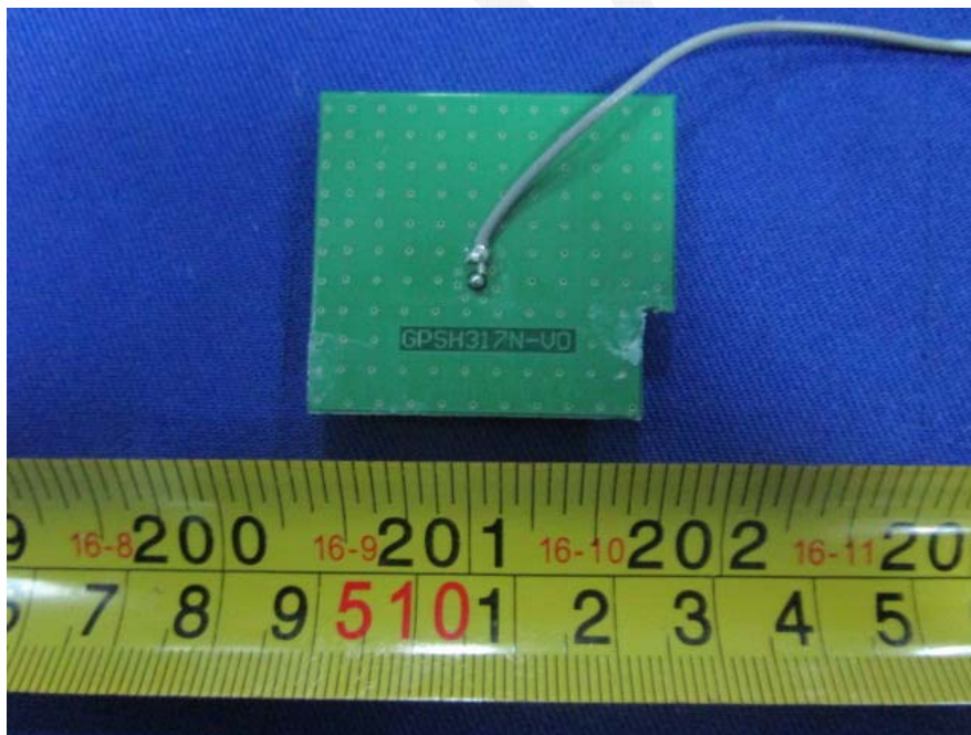
EUT -2.4G Antenna Bottom View
