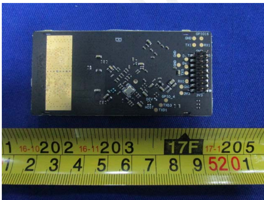
EUT -2.4GHz Module Bottom View
