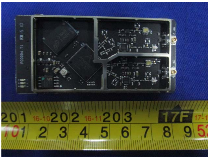
EUT -2.4GHz Module Top Unsheilded View
