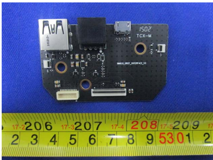
EUT –Port Top View
