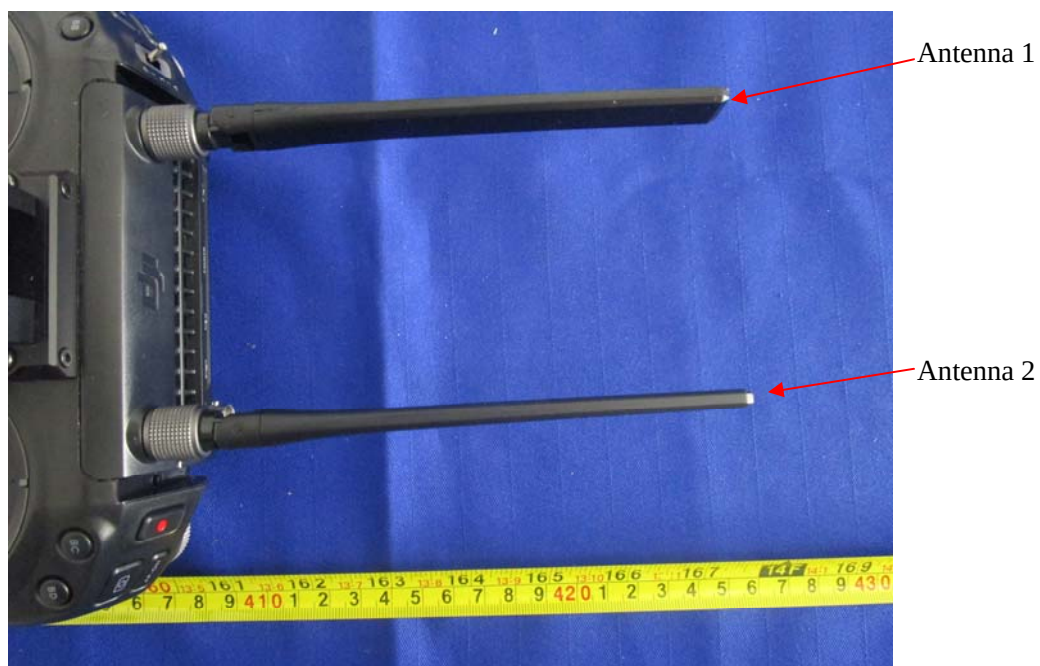
EUT – LB Antenna View
