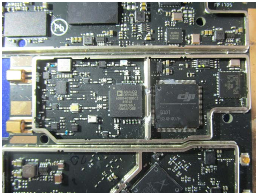
EUT – LB Module View
