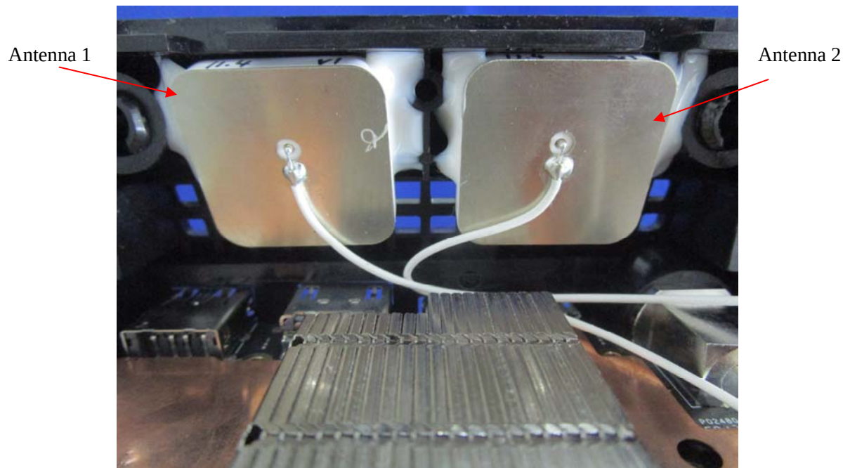
EUT – 10M Antenna View
