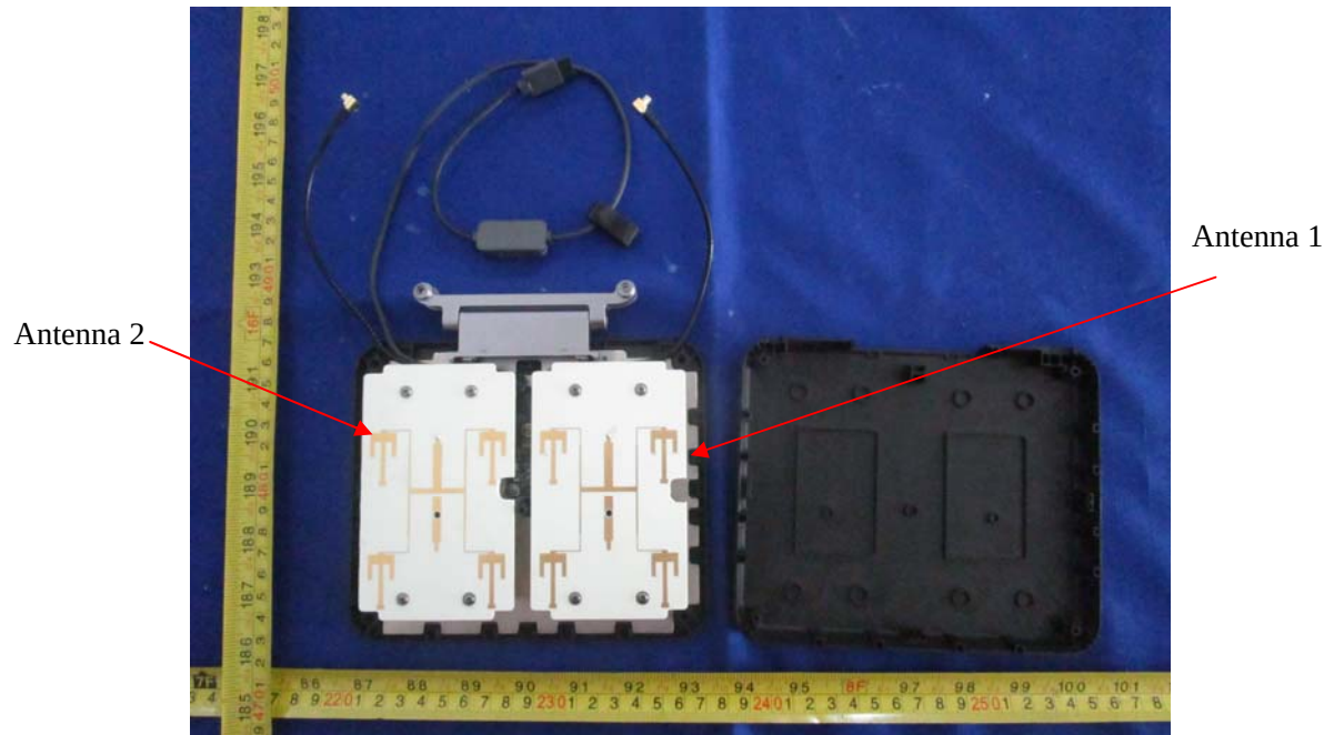
EUT – Antenna Case Open View
