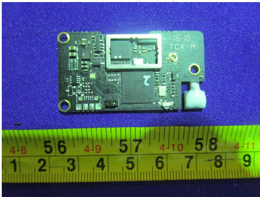
EUT – Main Board Unshield View
