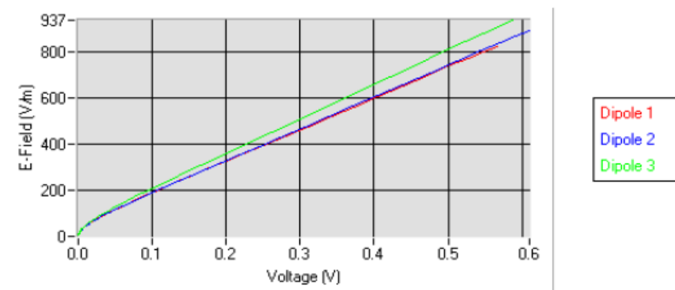
Calibration curves
