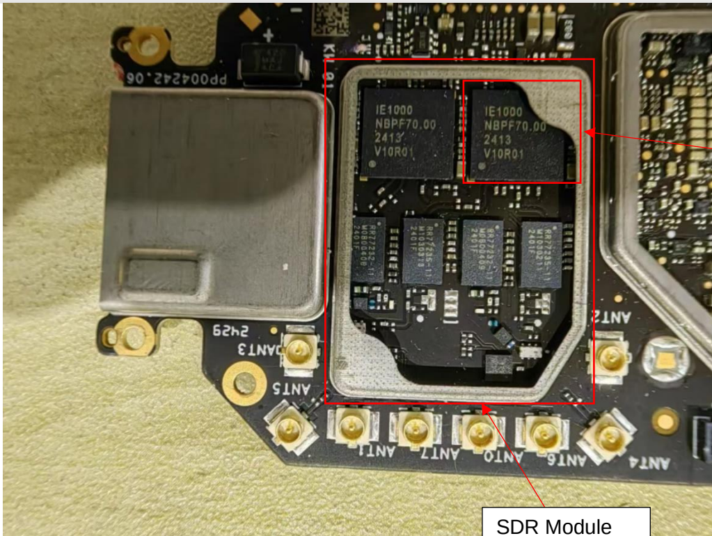
Internal View of EUT-36
