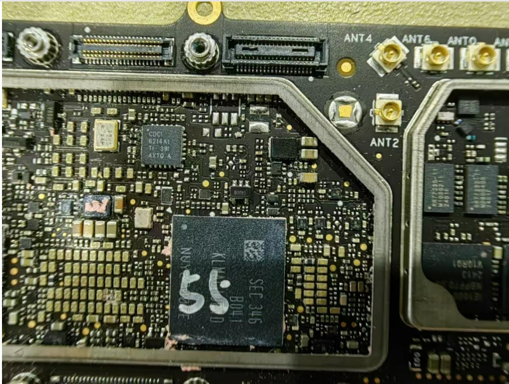
Internal View of EUT-35
