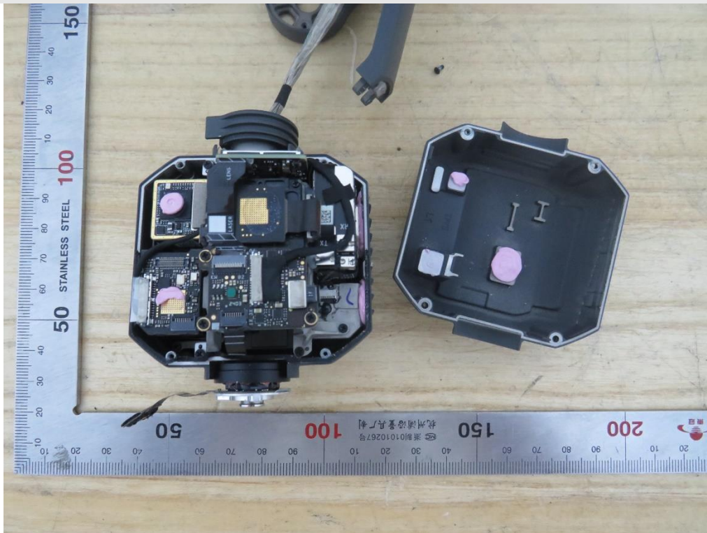
Internal View of EUT-130
