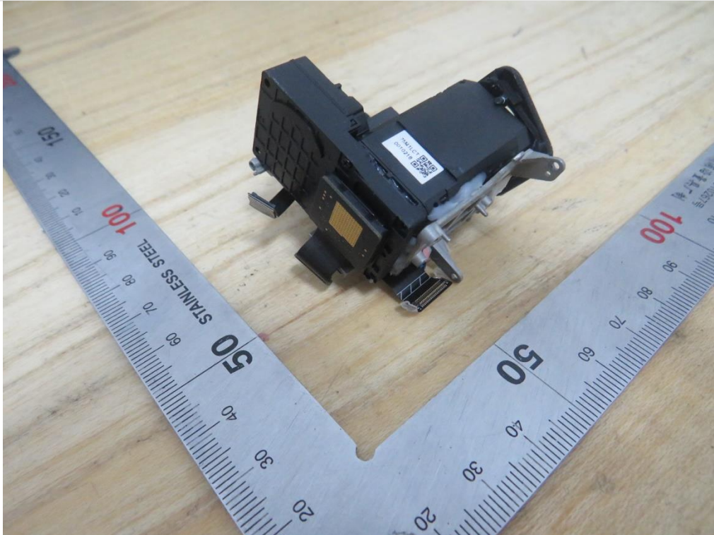
Internal View of EUT-140
