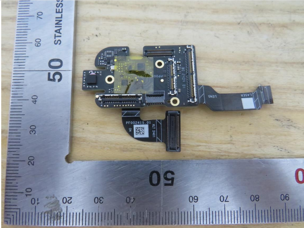
Internal View of EUT-132
