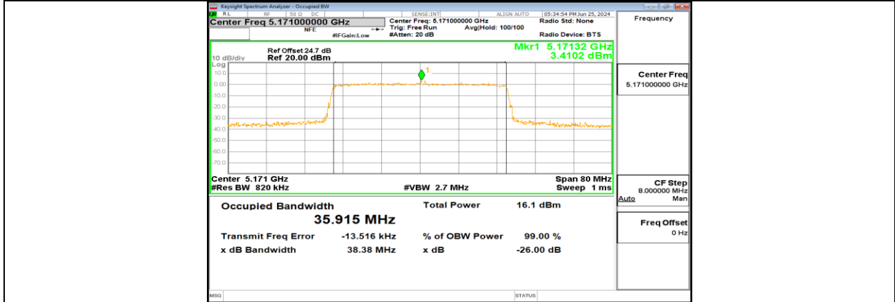
SRD 40MHz_Ant1_5171
