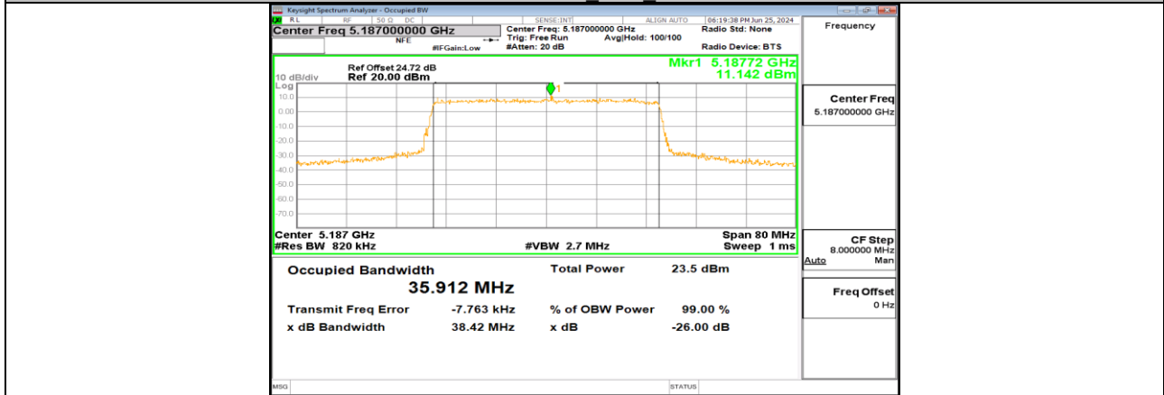
SRD 40MHz_Ant1_5187
