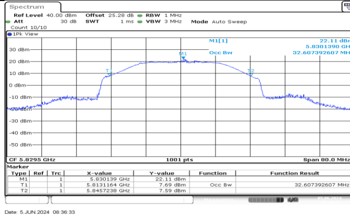
SRD 40MHz_Ant1_5829.5
