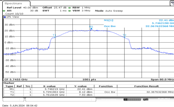
SRD 40MHz_Ant1_5745.5
