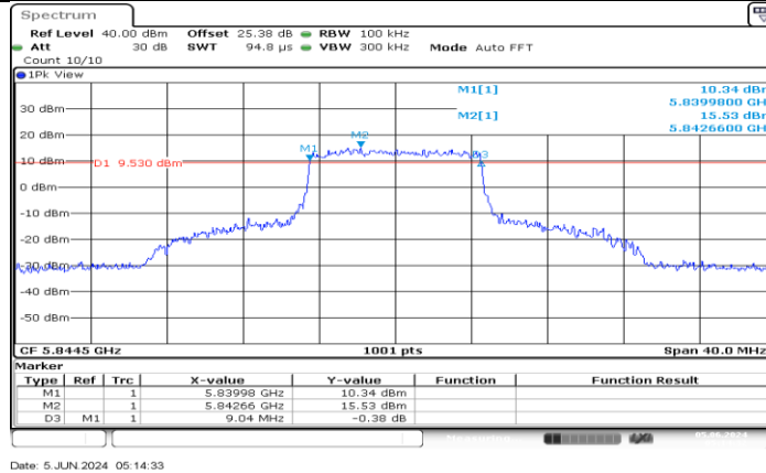
SRD 10MHz_Ant1_5844.5
