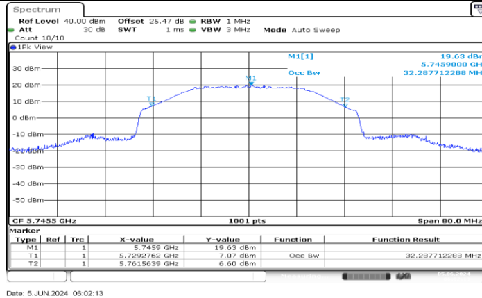
SRD 40MHz_Ant0_5745.5
