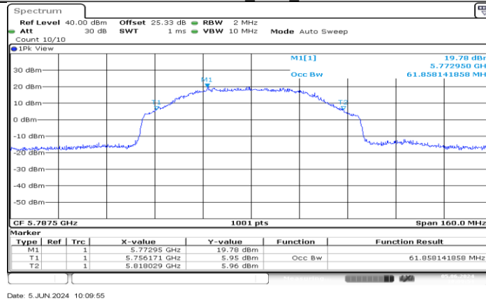
SRD 80MHz_Ant1_5787.5
