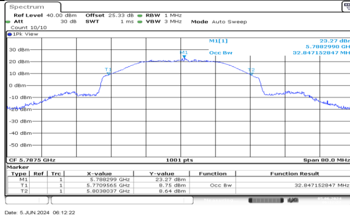
SRD 40MHz_Ant1_5787.5
