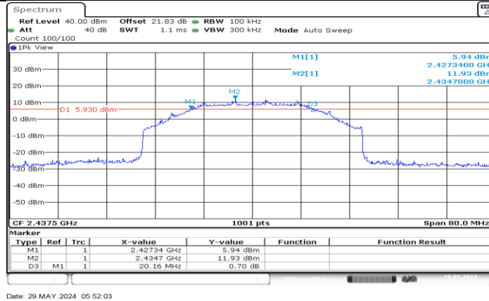
SRD 40MHz_Ant0_2437.5
