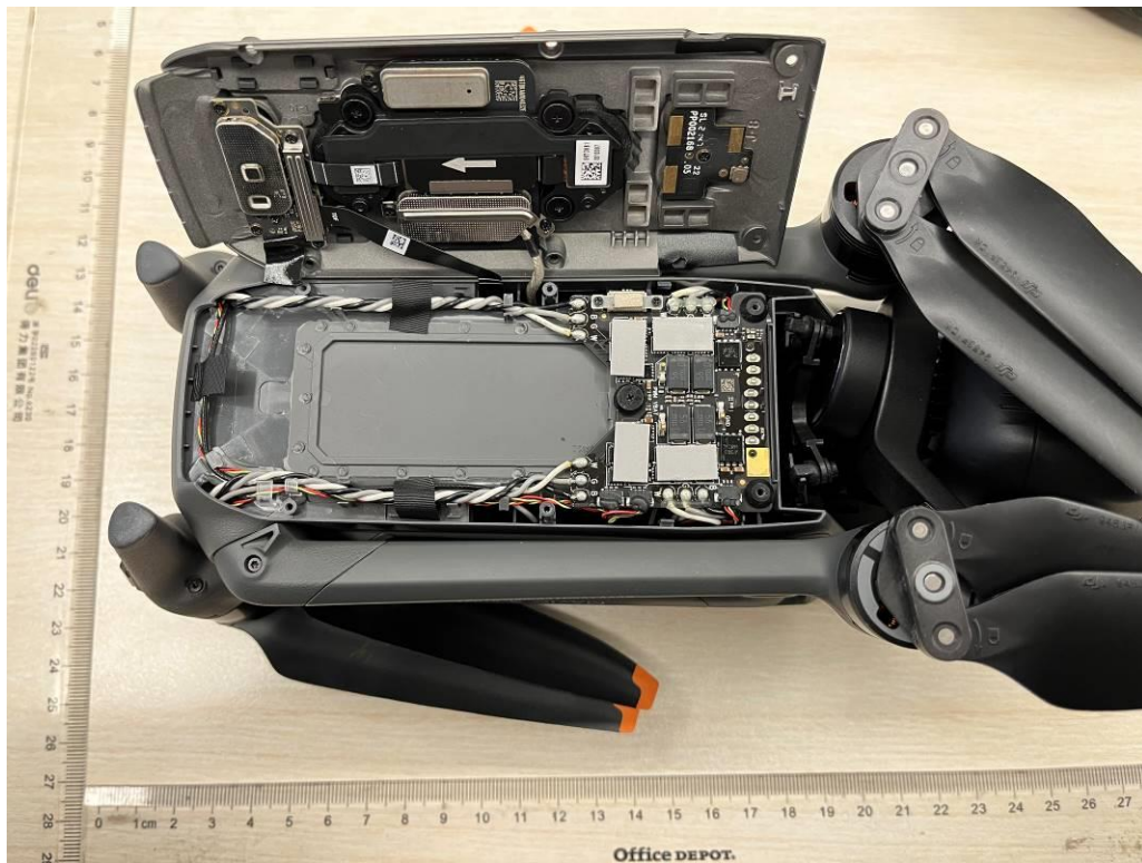
Figure 13: Internal view 5 (with bottom cover opened)
