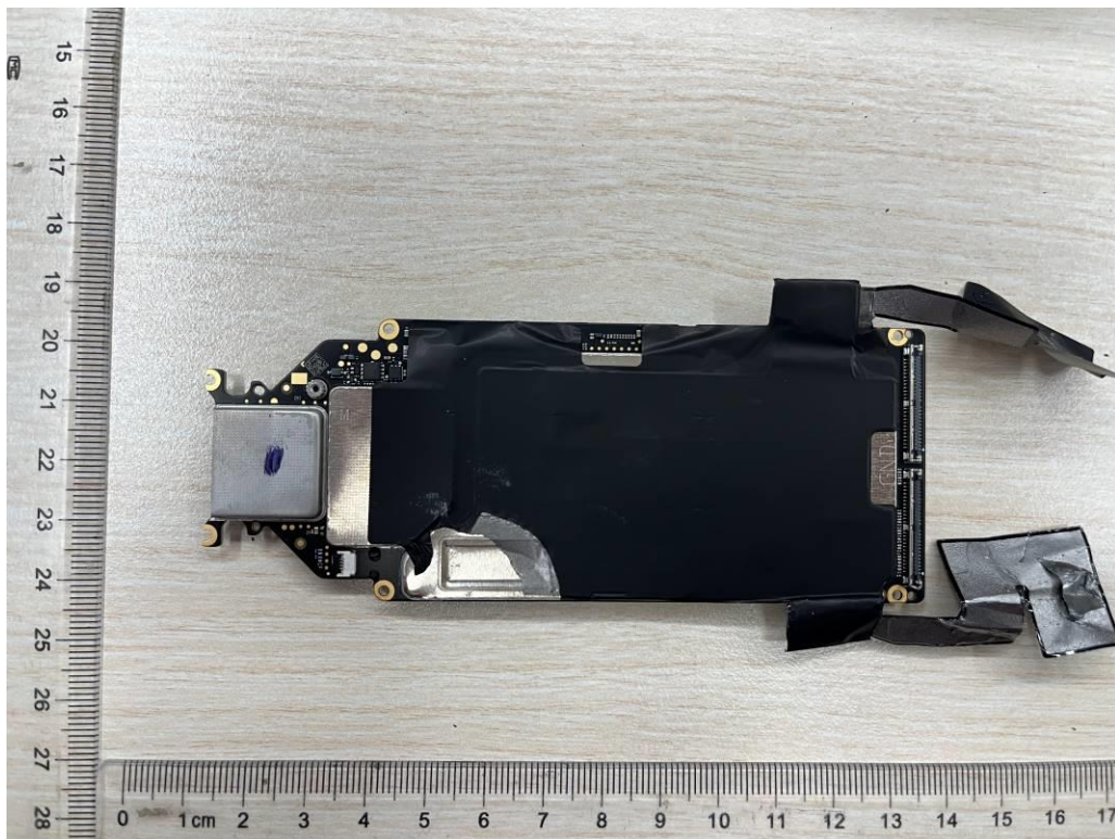
Figure 12: Mainboard view 3
