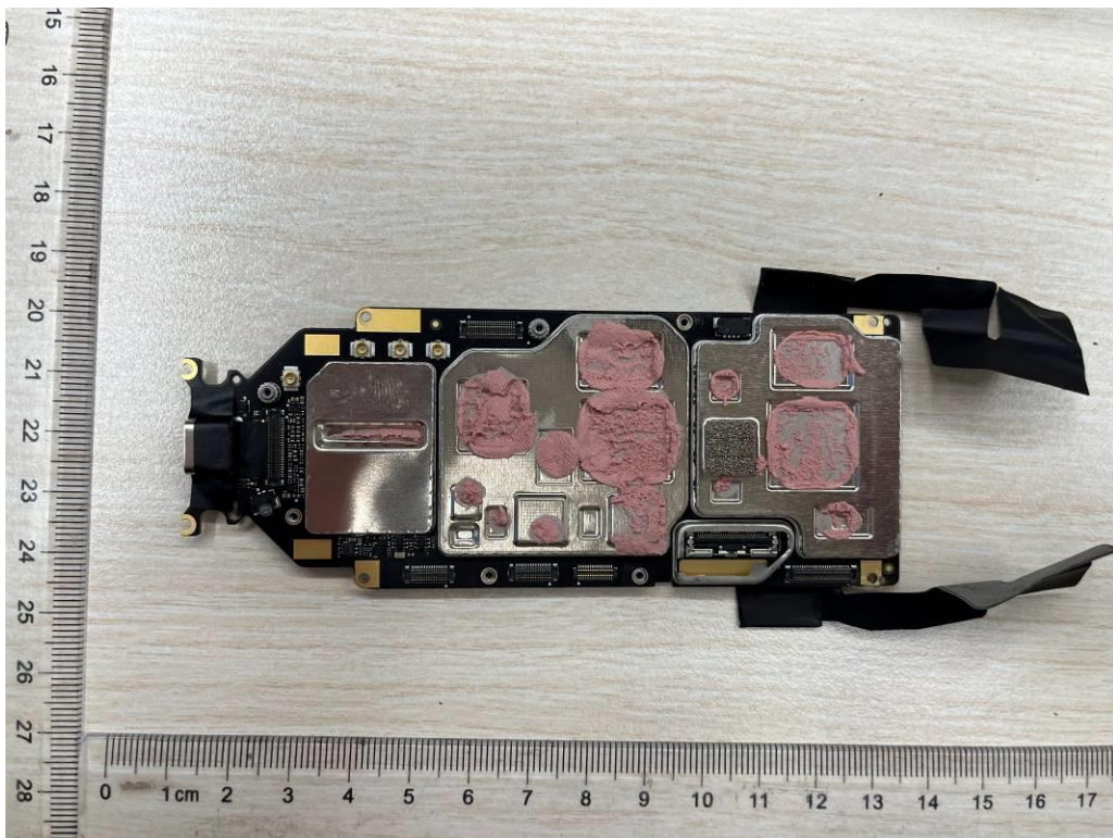
Figure 10: Mainboard view 1
