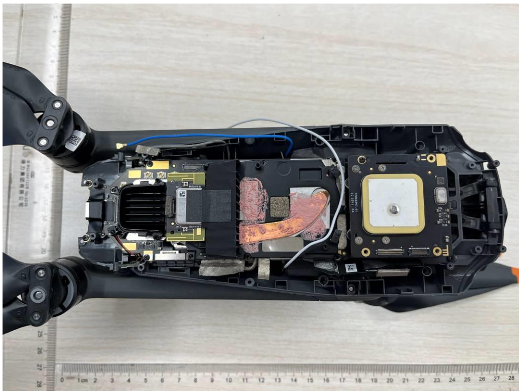
Figure 8: View with DC fan removed
