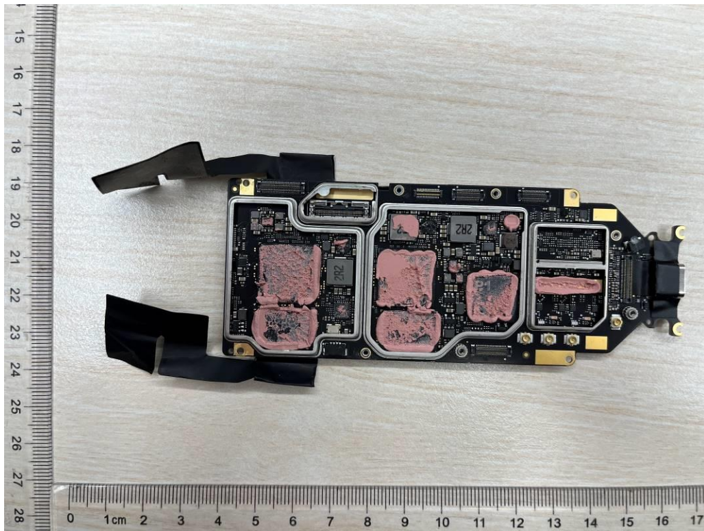
Figure 11: Mainboard view 2
