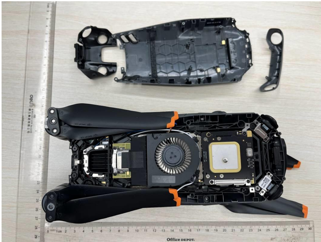
Figure 5: Internal view 1
