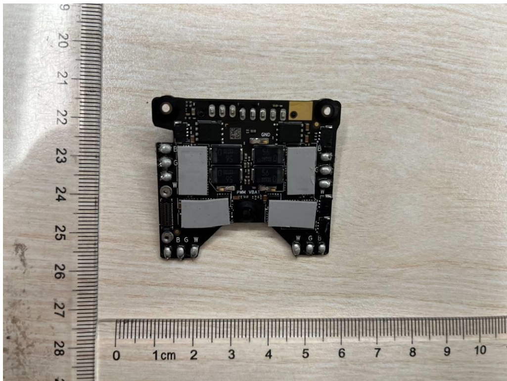
Figure 14. Battery board view 1
