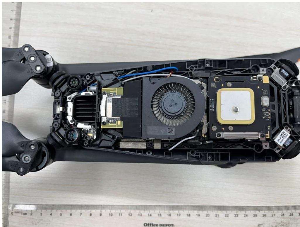
Figure 6: Internal view 2
