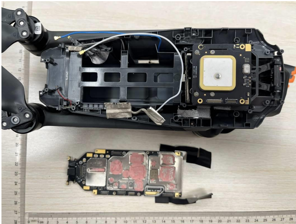
Figure 9: Internal view 4
