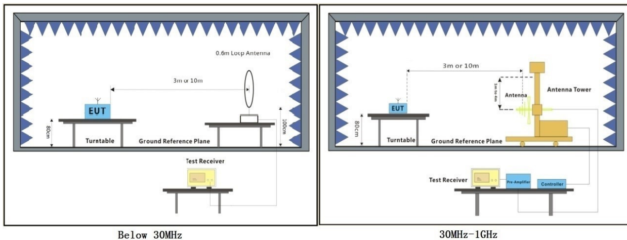
Below 30MHz
