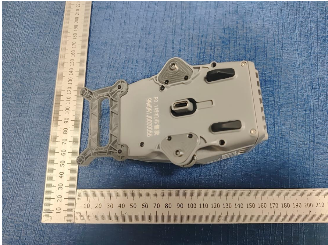
Fig.3. External view
