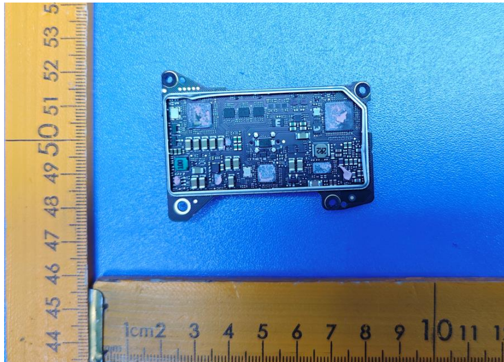
Fig.10. PCB view
