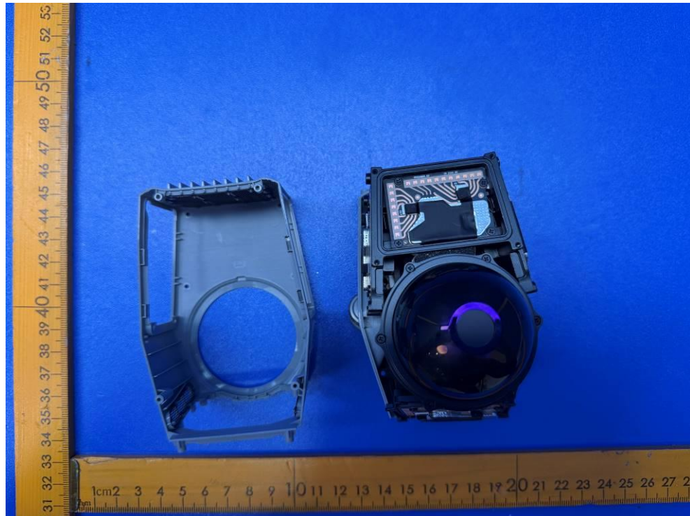
Fig.5. Internal view
