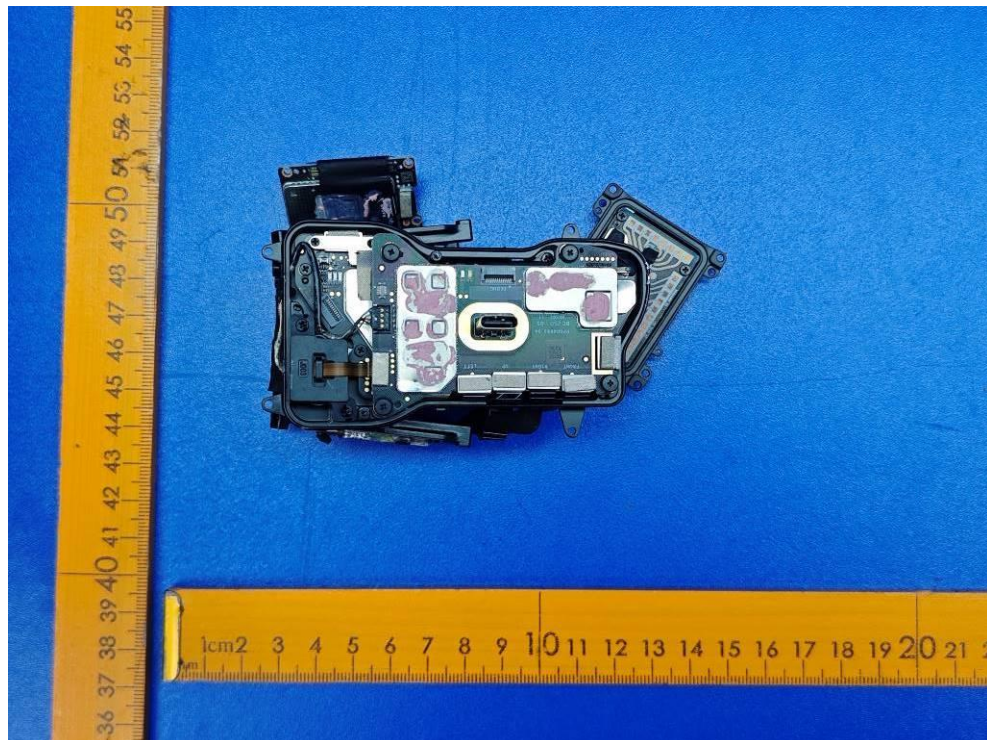
Fig.6. Internal view
