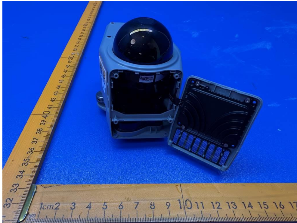
Fig.3. Internal view
