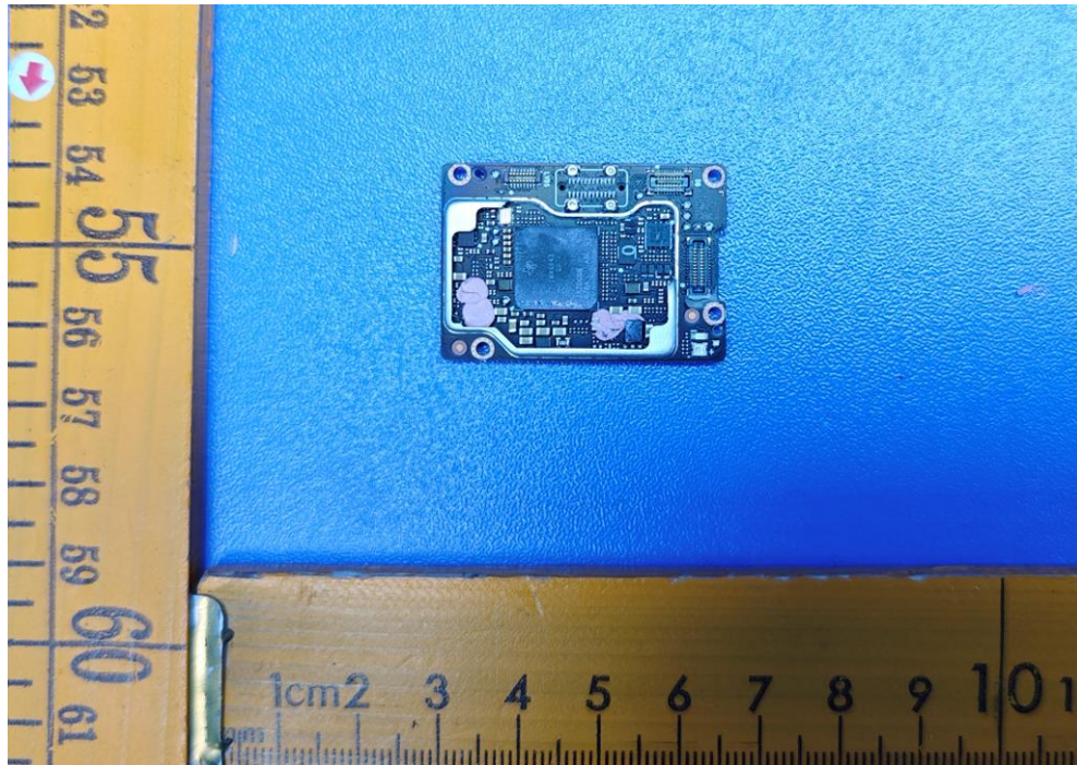
Fig.7. PCB view
