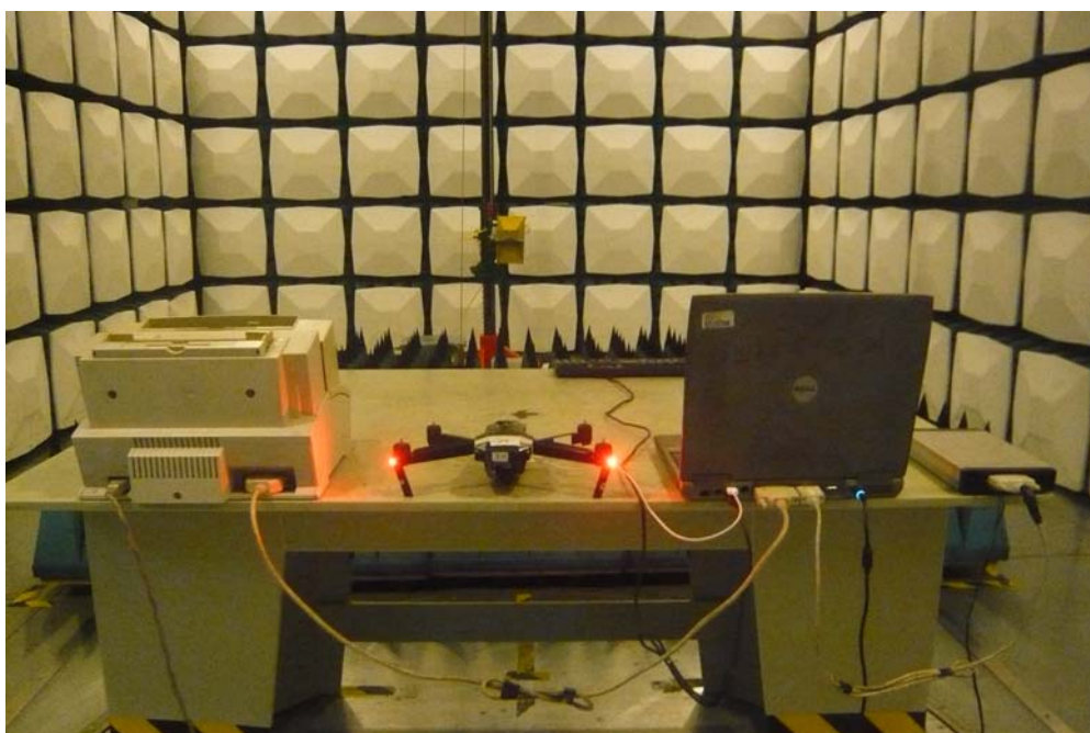
Radiated Emission View-Back (Above 1GHz)
