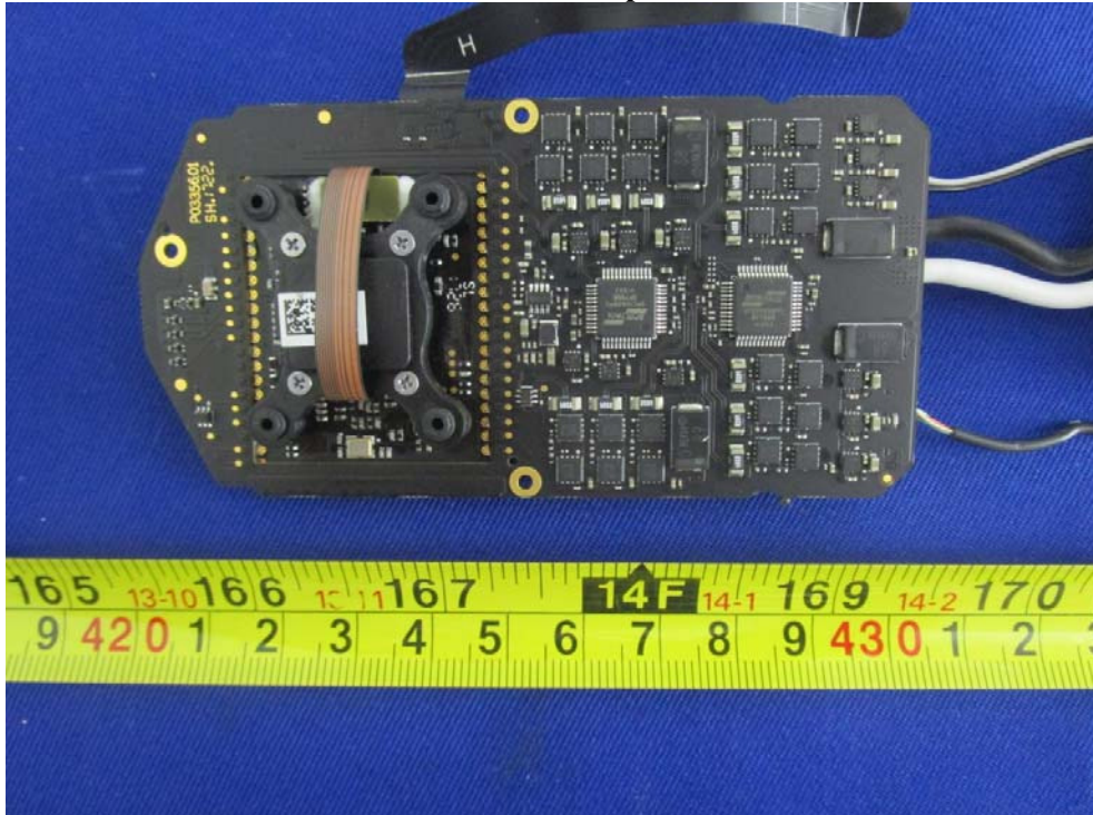
EUT – Board2 Top View
