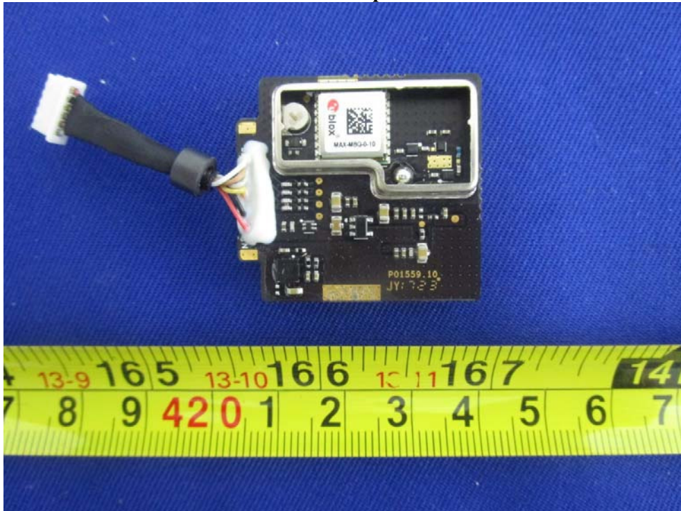
EUT – GPS Module Top Unshield View
