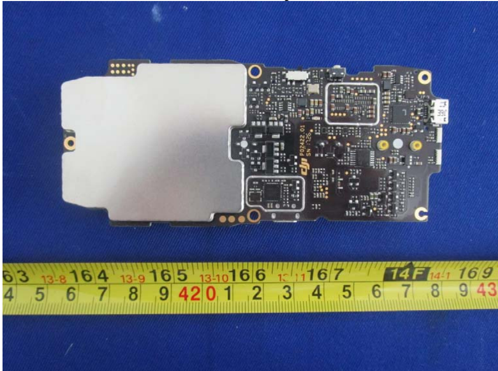
EUT – Board1 Top View
