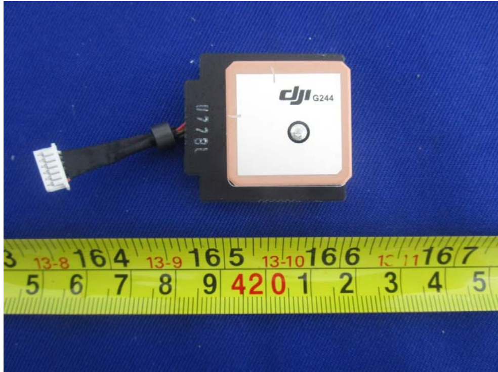
EUT – GPS Module Bottom View
