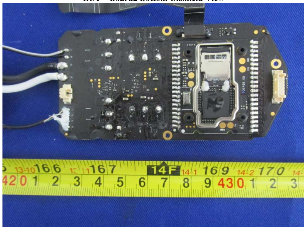
EUT – Board2 Bottom Unshield View
