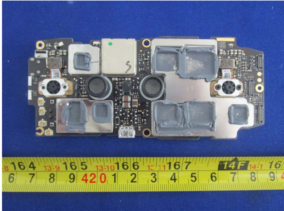
EUT – Board1 Bottom View
