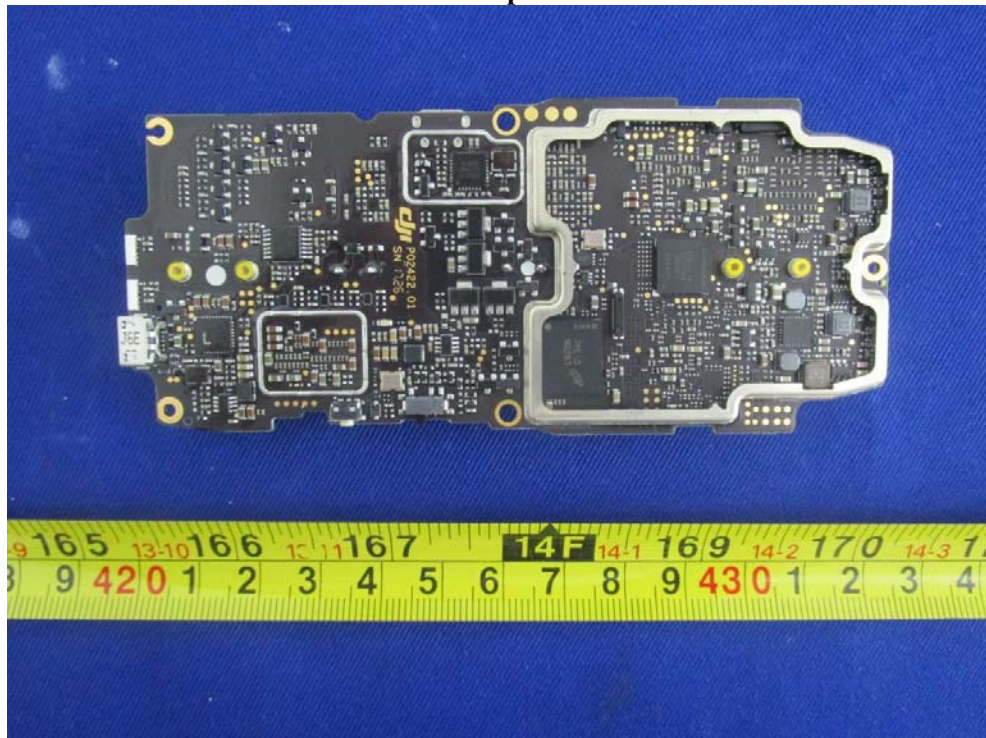
EUT – Board1 Top Unshield View
