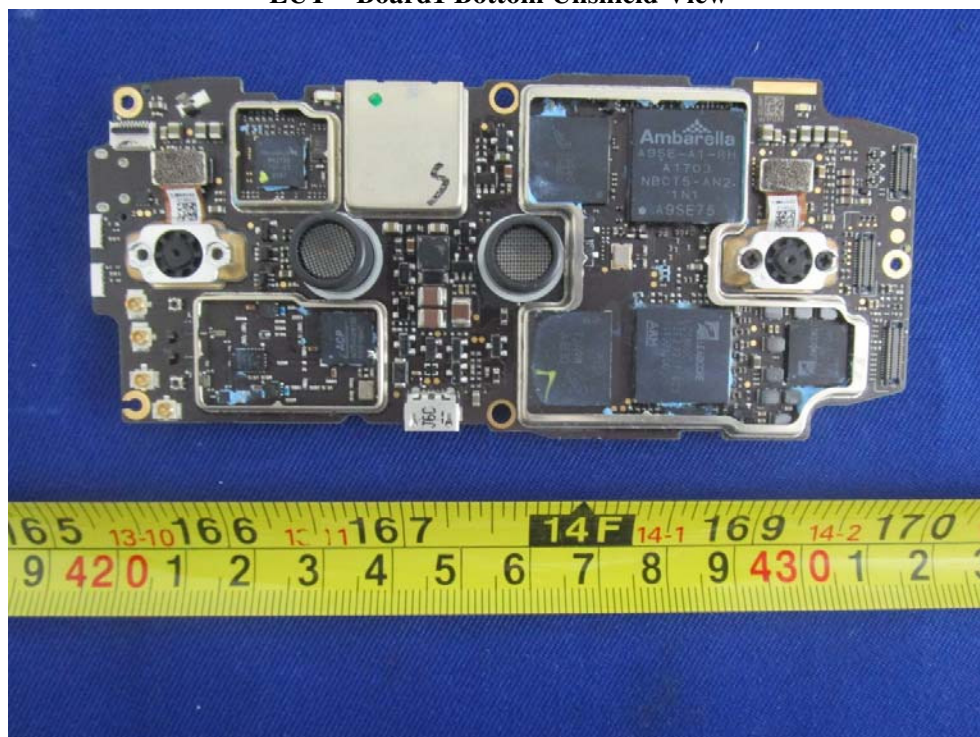
EUT – Board1 Bottom Unshield View
