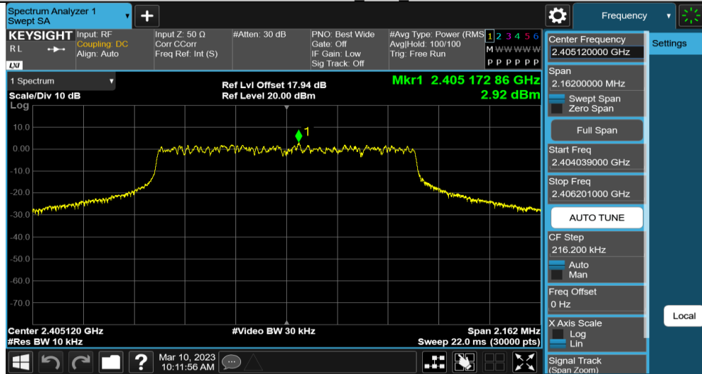
1.4MCA-MIMO Ant3 2405.12
