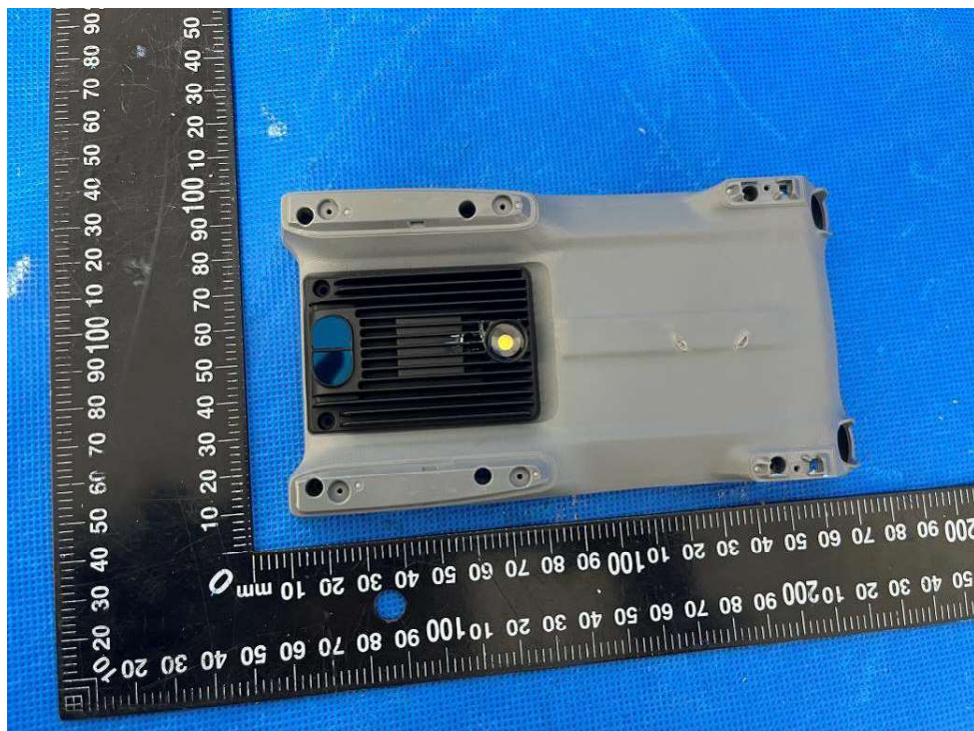
Fig.52. Bottom LED view
