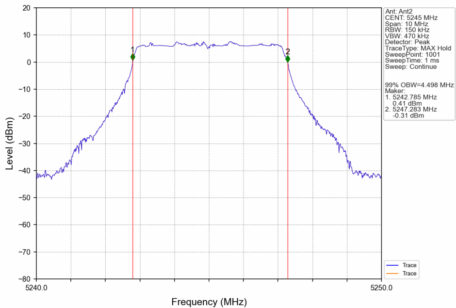
5M_HCH_5245MHz_Ant2_NTNV
