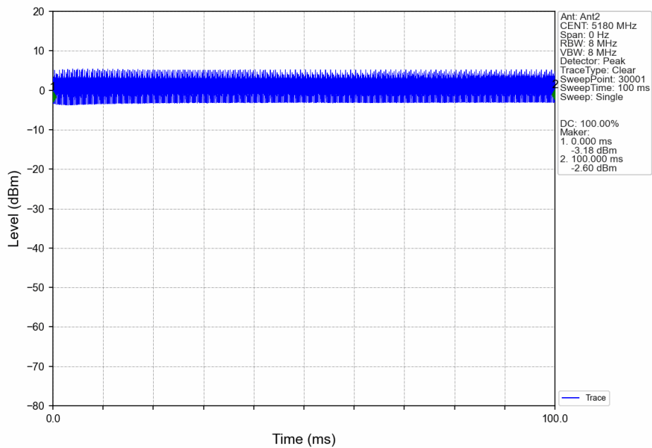
60M_LCH_5180MHz_Ant2_NTNV
