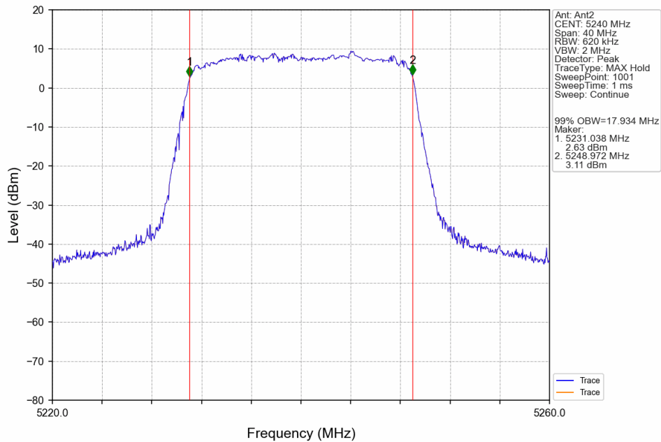
20M_HCH_5240MHz_Ant2_NTNV
