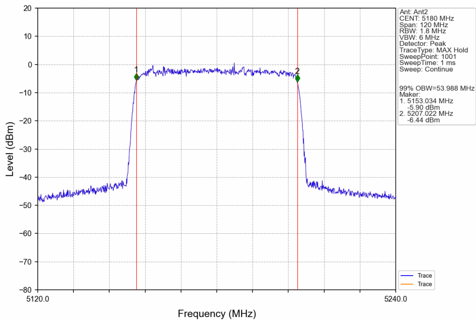
60M_LCH_5180MHz_Ant2_NTNV
