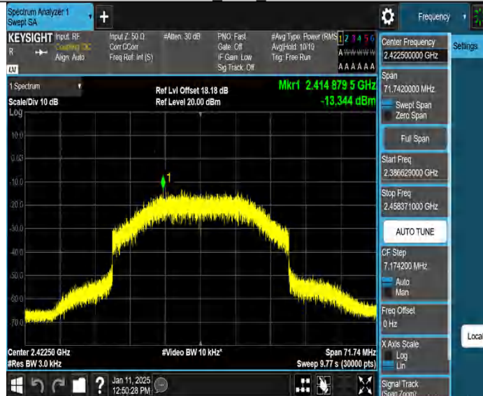
40M_Ant5_2422.5
