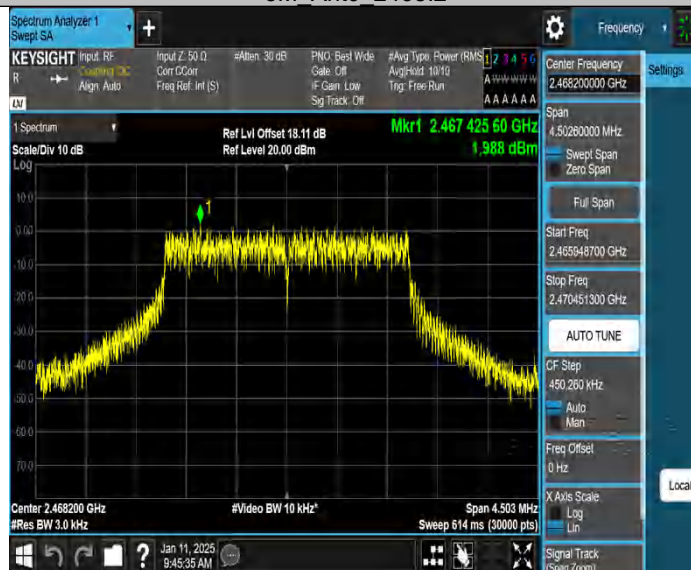
3M_Ant5_2468.2
