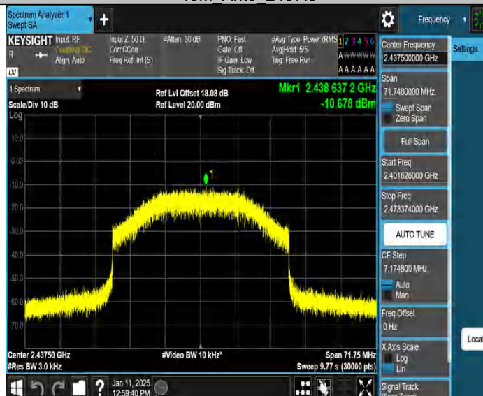
40M_Ant0_2437.5
