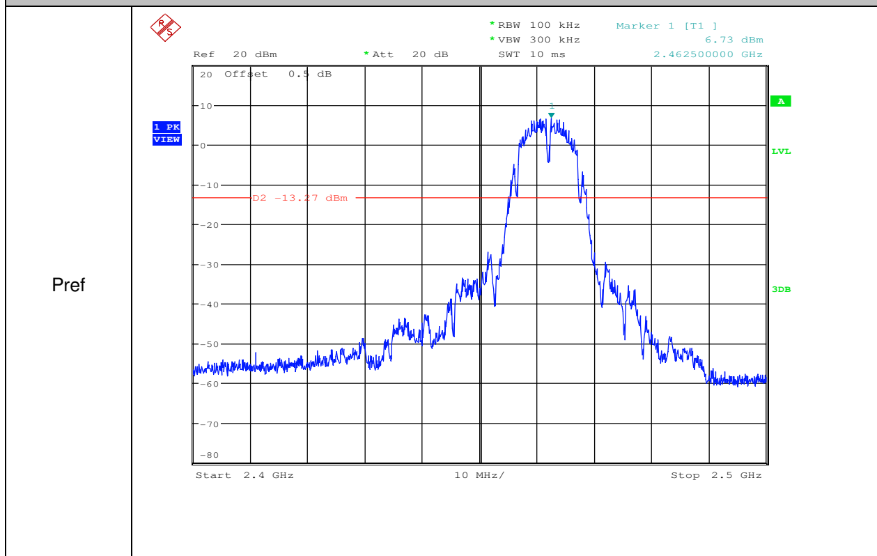
RF Conducted Spurious Emissions_11B_2462_Ant2
