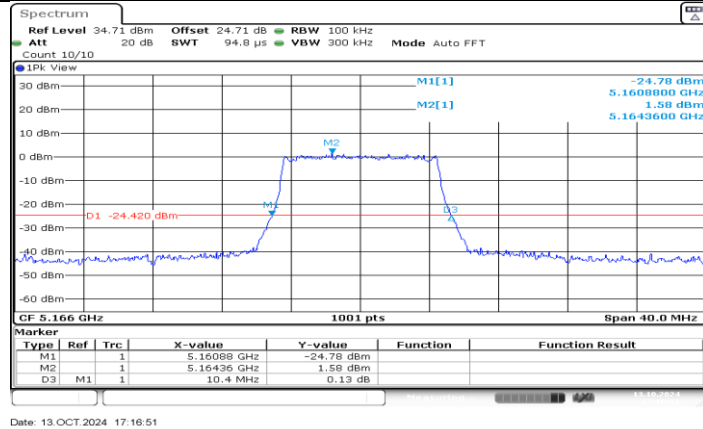
SRD 10M_Ant1_5166
