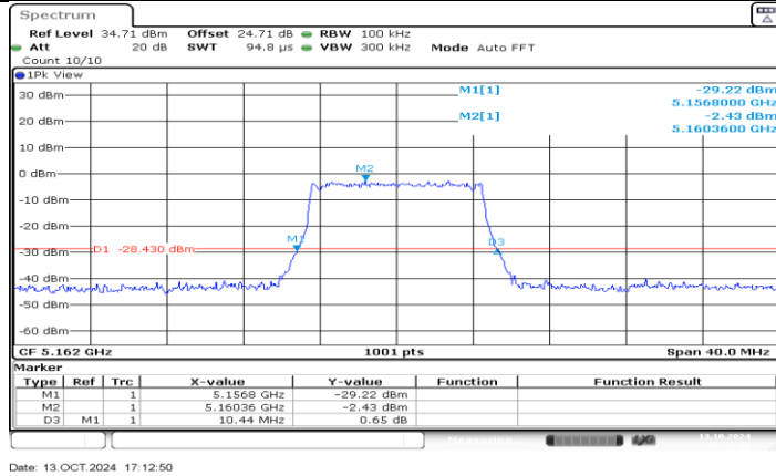
SRD 10M_Ant1_5162
