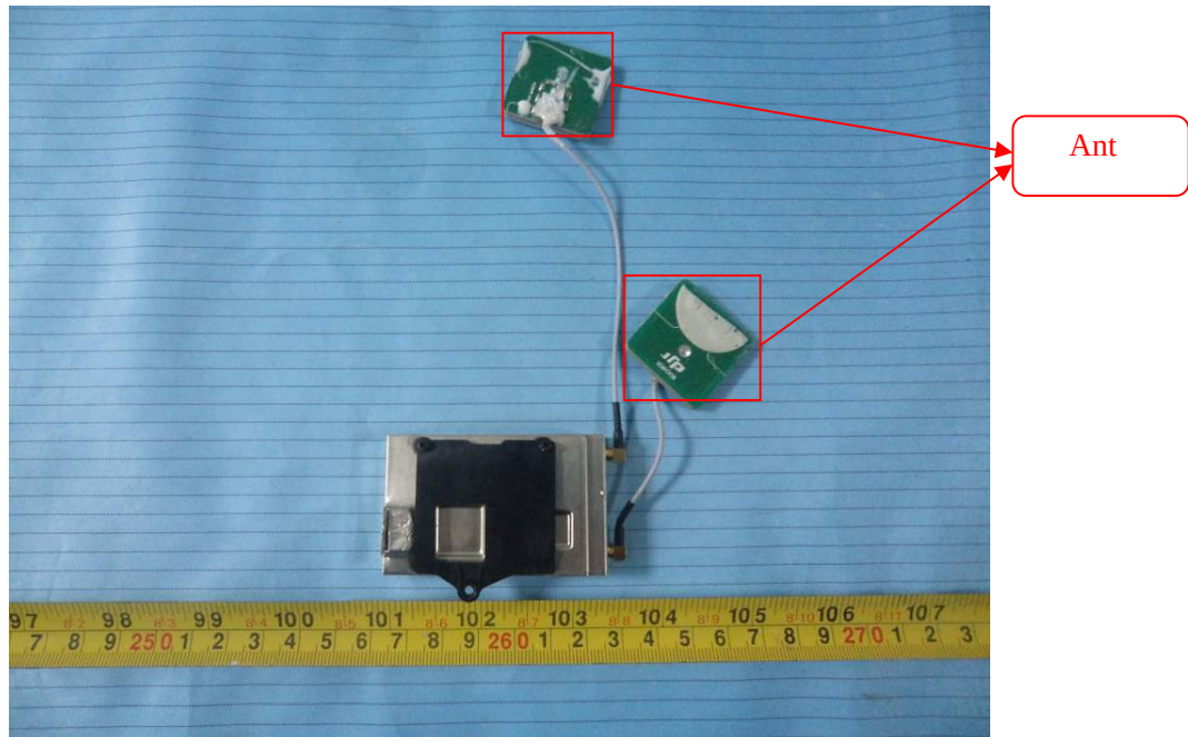
EUT – 2.4G Wifi Module Bottom View
