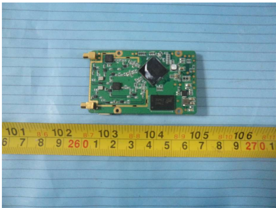
EUT – 2.4G Wifi Module Board 2 Top Shielding off View
