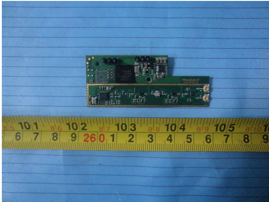
EUT – 5.8G Module Board Top View
