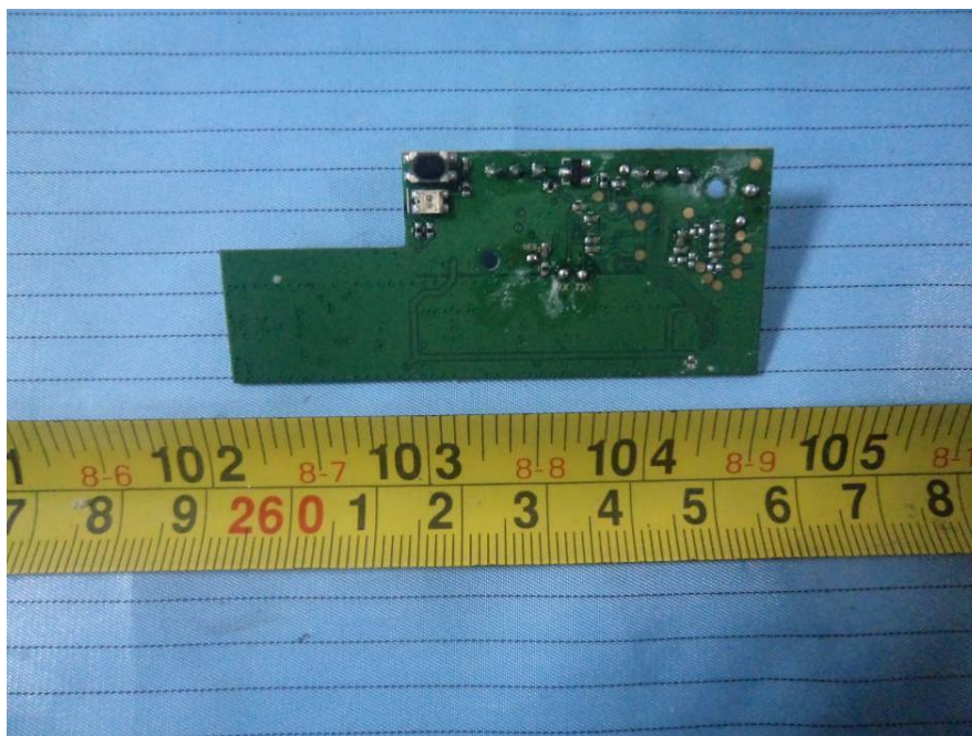
EUT – 5.8G Module Board Bottom View
