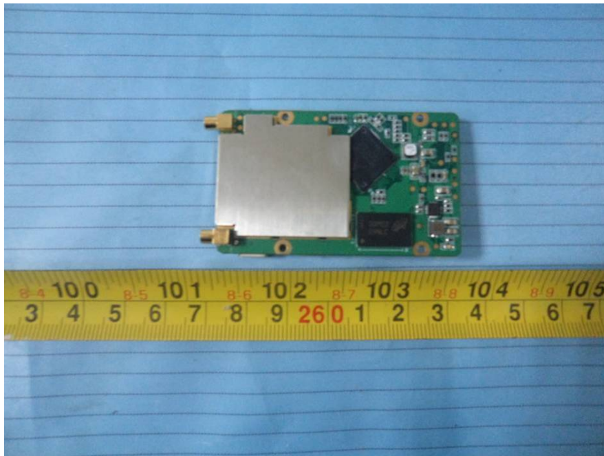
EUT – 2.4G Wifi Module Board 2 Top View
