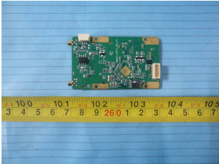
EUT – 2.4G Wifi Module Board 2 Bottom View
